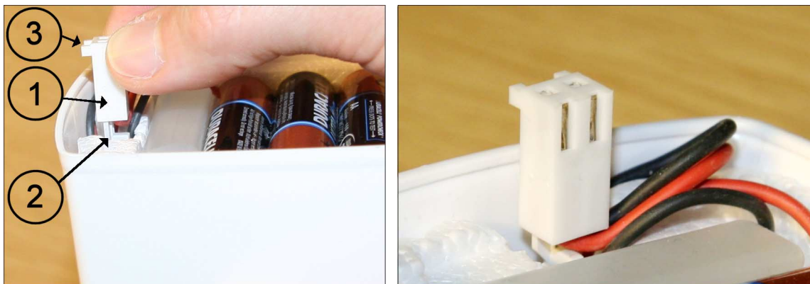
Figure 24 Placing Battery Connector into Connector Holder, Part 2
