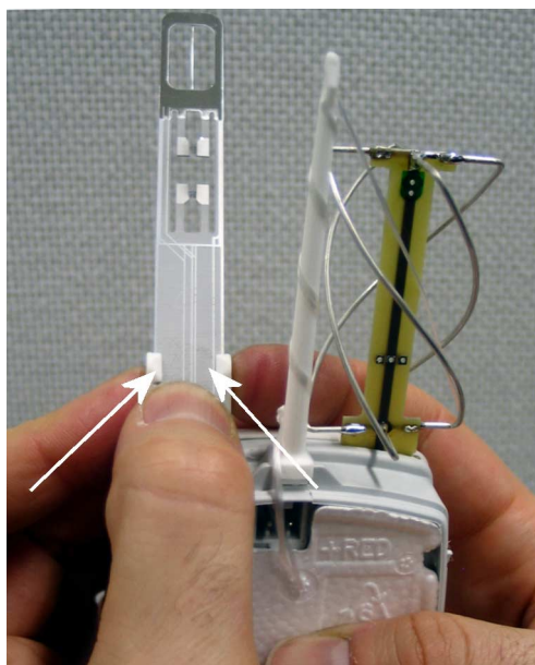
Figure 15 Placing the Sensor Boom into Flight Position
