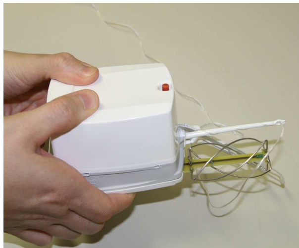
Figure 26 Pressing Battery Case and Radiosonde Together
