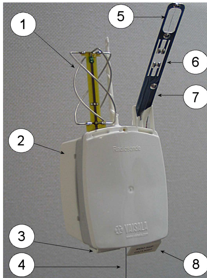
Figure 1 Vaisala Radiosonde RS92-SGP
