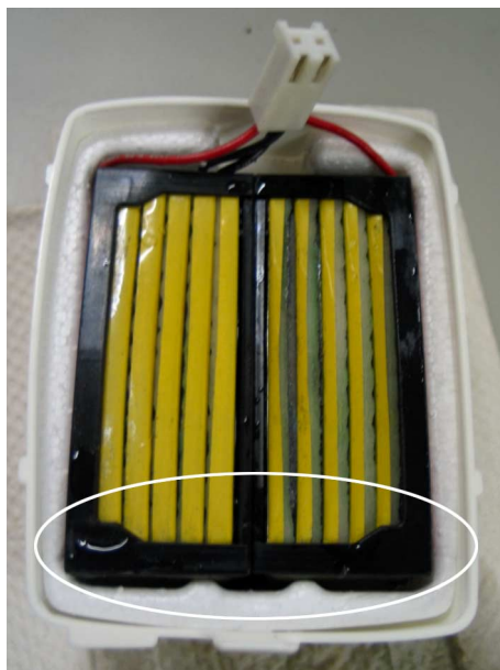
Figure 30 Battery in the Case, Waxed End Circled
