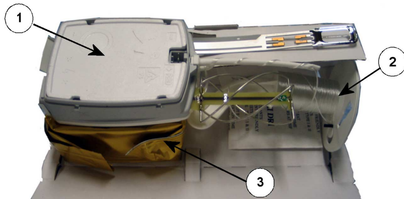
Figure 11 Contents of the Radiosonde Package
