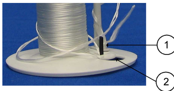
Figure 12 Unwinder Details
