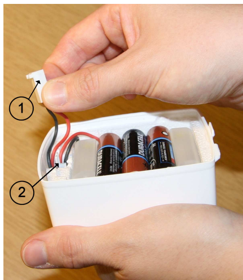
Figure 23 Placing Battery Connector into Connector Holder, Part 1
