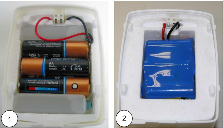
Figure 16 RSB511 Dry-cell Battery Set (Number 1) and RSB611 Lithium Battery (Number 2)
