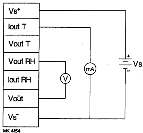
Fig. 5 Recommended connection when the output signals for temperature and humidity are not of the same type
