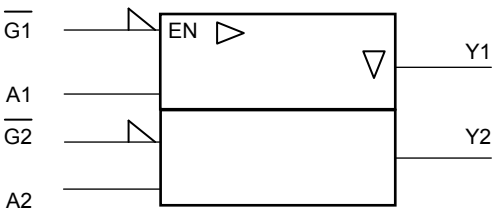
IEC Logic Symbol
