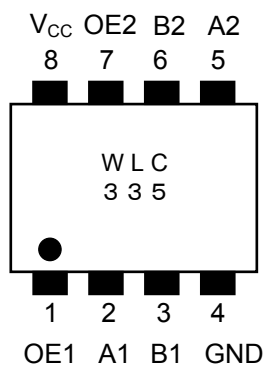
TC7WBL3305CFK
