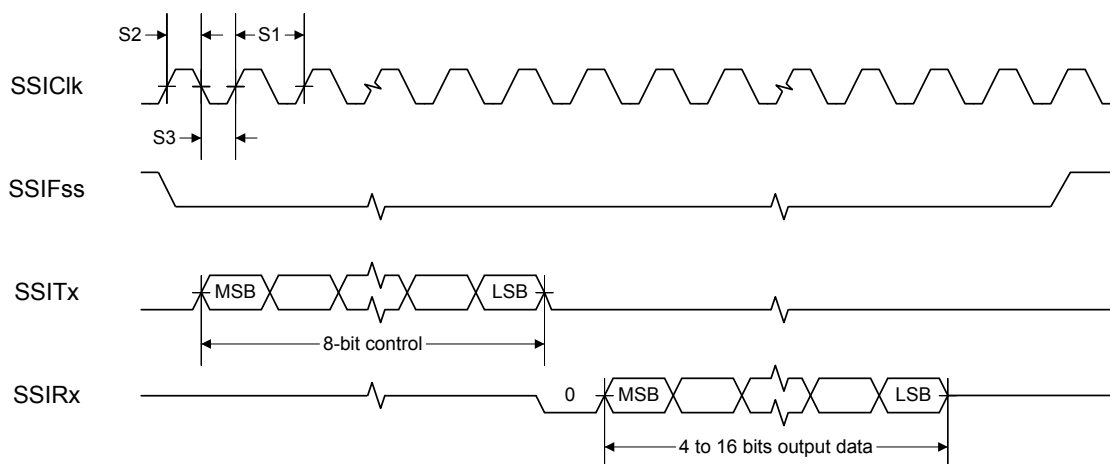
Figure 19-3. SSI Timing for MICROWIRE Frame Format (FRF=10), Single Transfer
