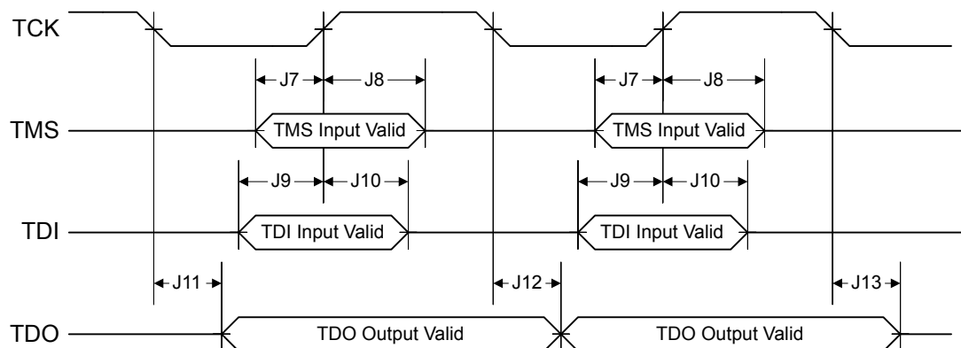
Figure 19-6. JTAG Test Access Port (TAP) Timing
