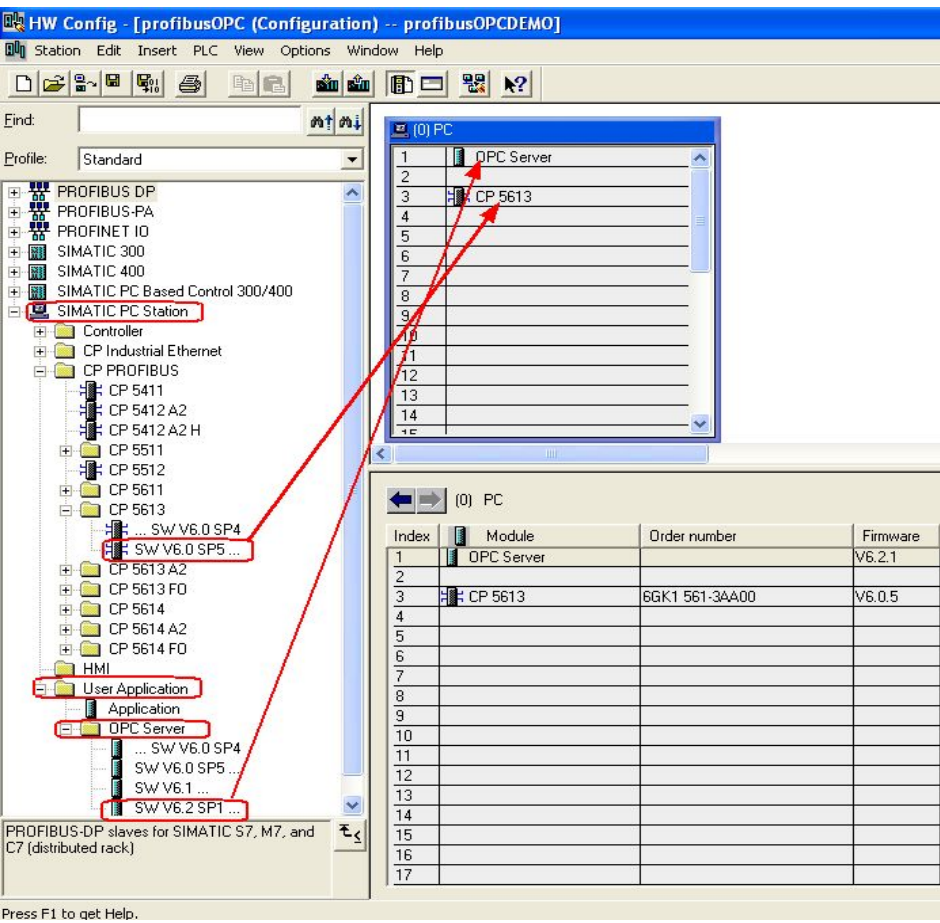
图 11: PC Station 硬件组态
