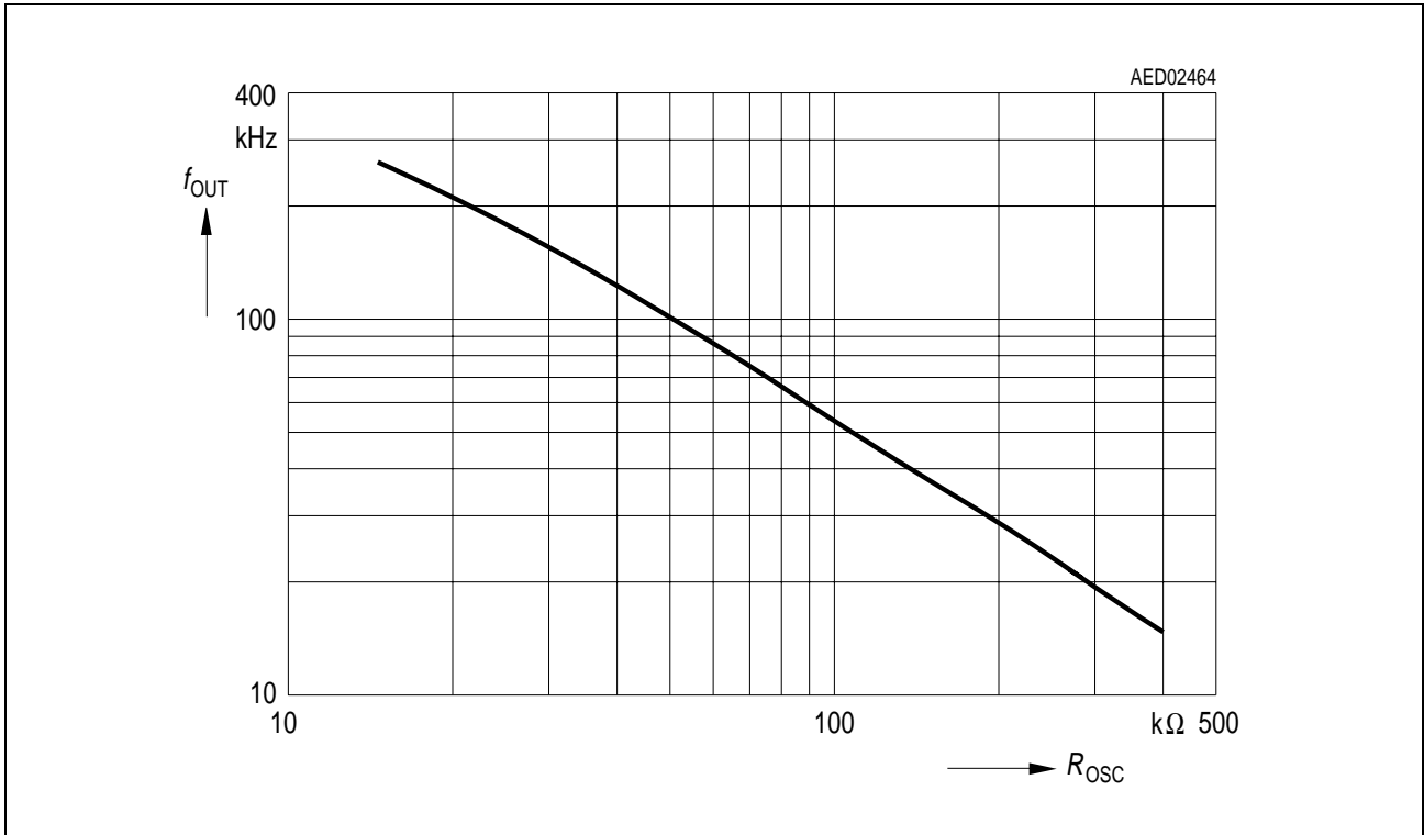
Figure 5 PFC/PWM Frequency
