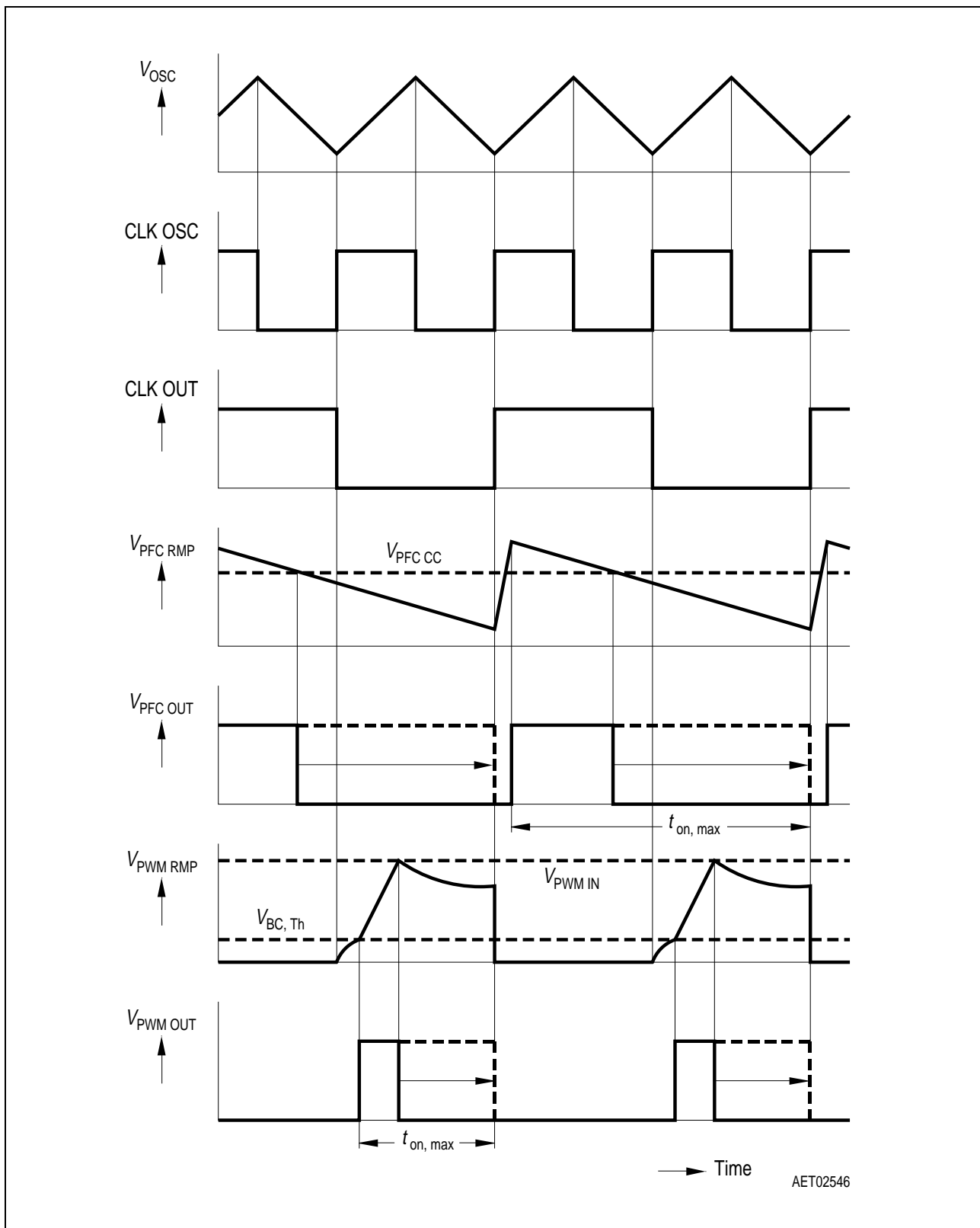
Figure 18 Timing Diagram without Synchronization
