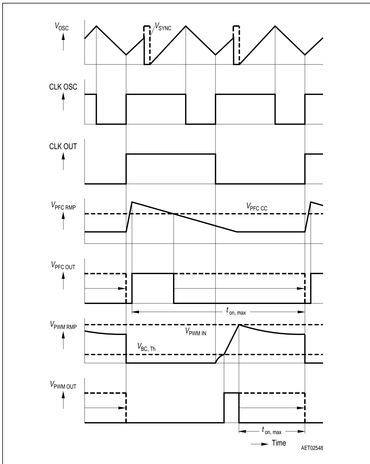
Figure 20 Timing Diagram with Synchronization ( f_{SYNC} < f_{osc} )
