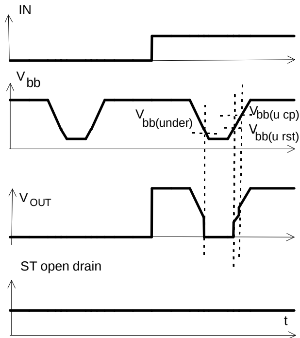
Figure 6a: Undervoltage:
