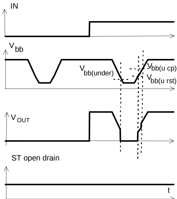
Figure 6a: Undervoltage:
