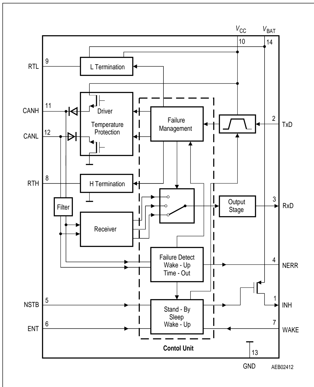
Figure 3 Block Diagram
