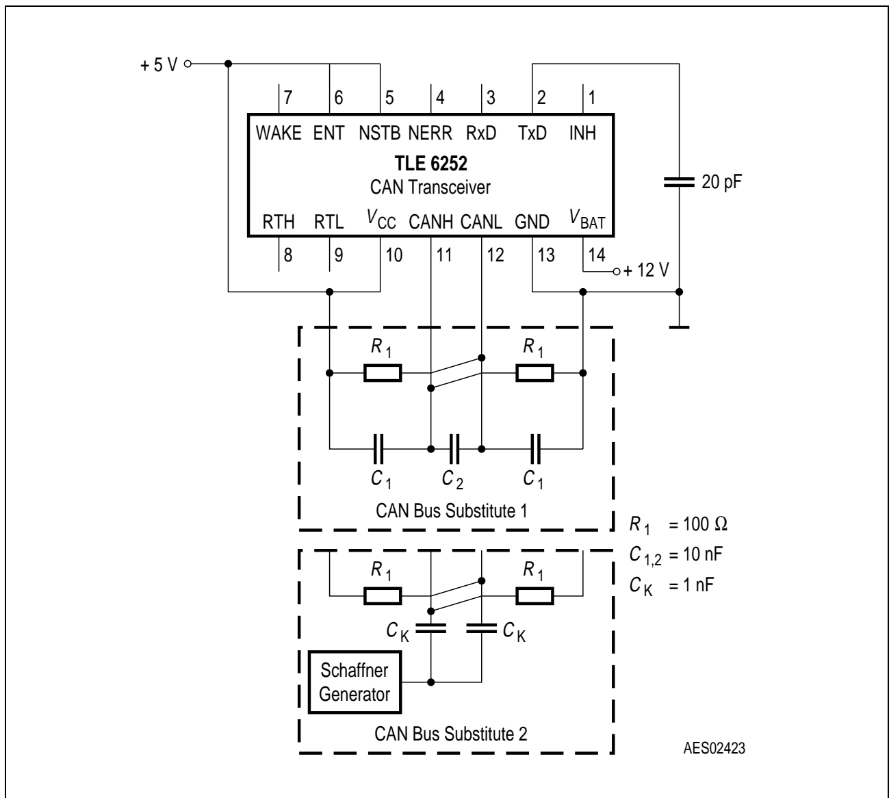
Figure 5 Test Circuits
