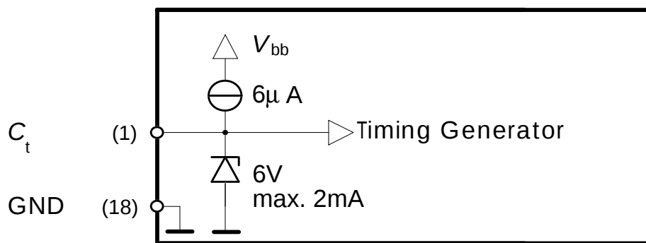
Triangular Waveform Generator Input C_t (1)
