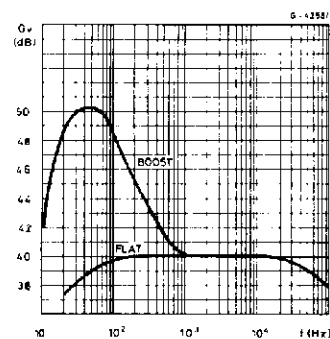
Figure 28. Frequency response of the circuit of fig. 27
