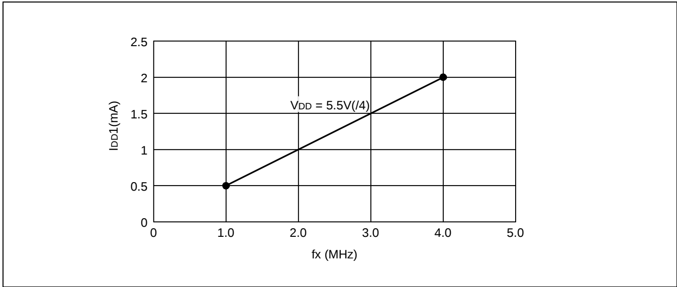
Figure 14-14. I_{DD} vs. Frequency
