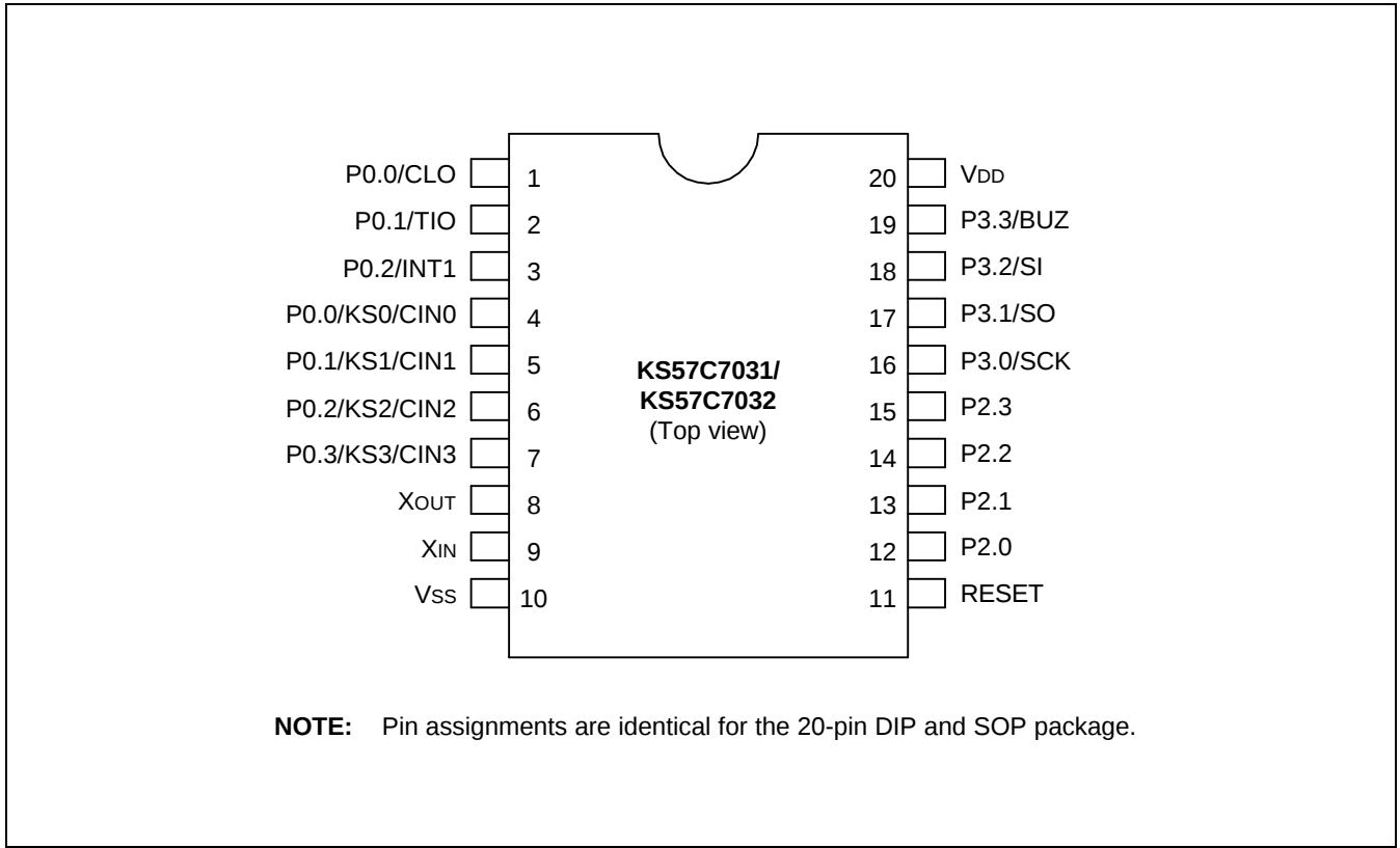
Figure 1-2. S3C7031/7032 Pin Assignment Diagram (20-pin DIP/SOP Package)
