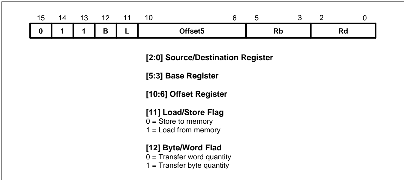
Figure 3-38. Format 9
