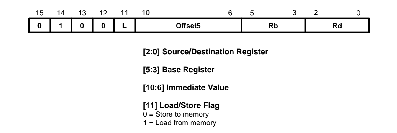
Figure 3-39. Format 10
