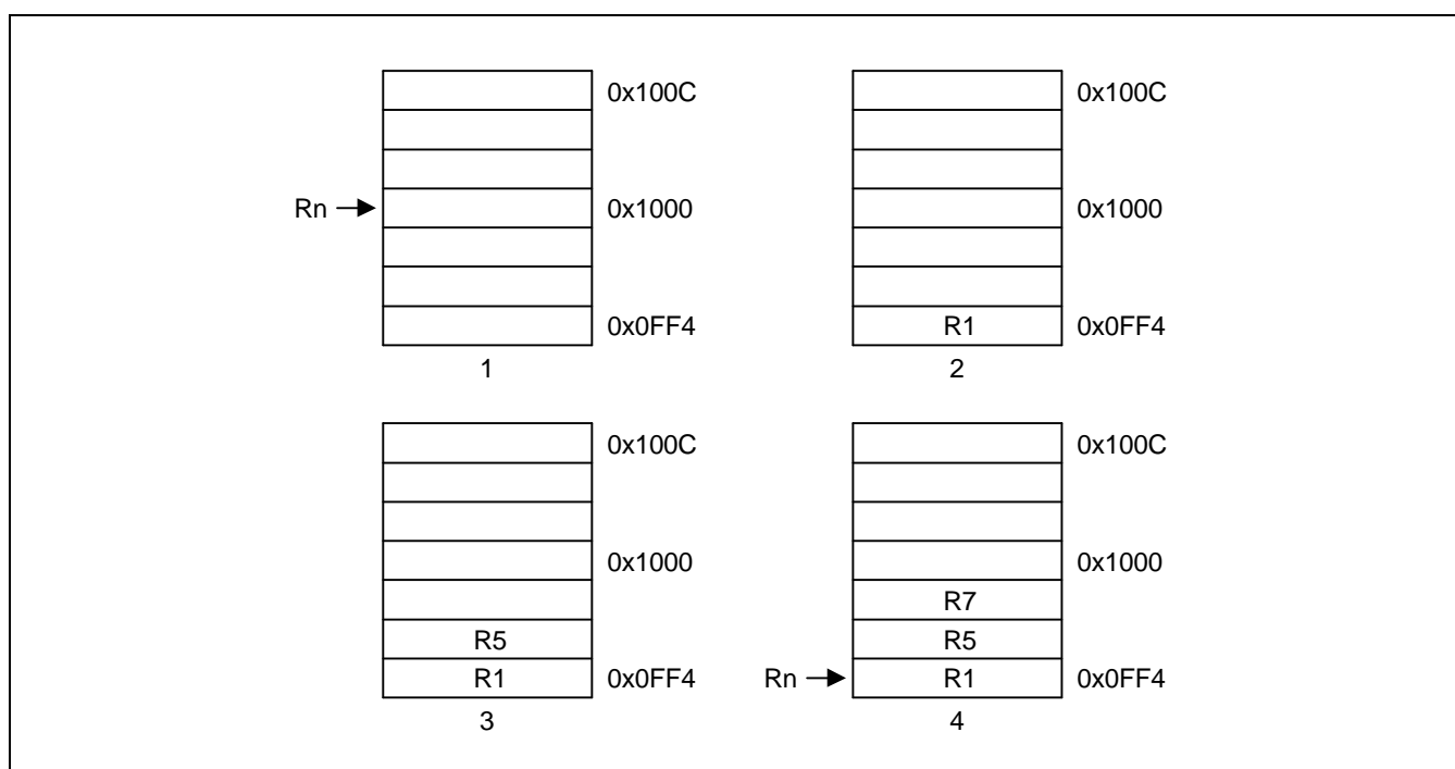
Figure 3-22. Pre-Decrement Addressing
