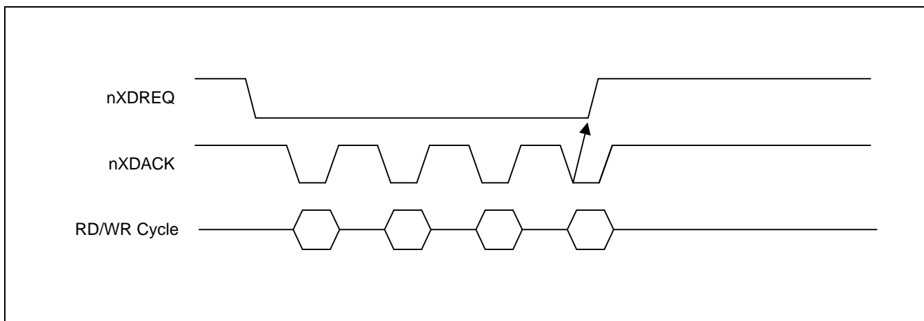
Figure 9-7. External DMA Requests (Demand Mode)
