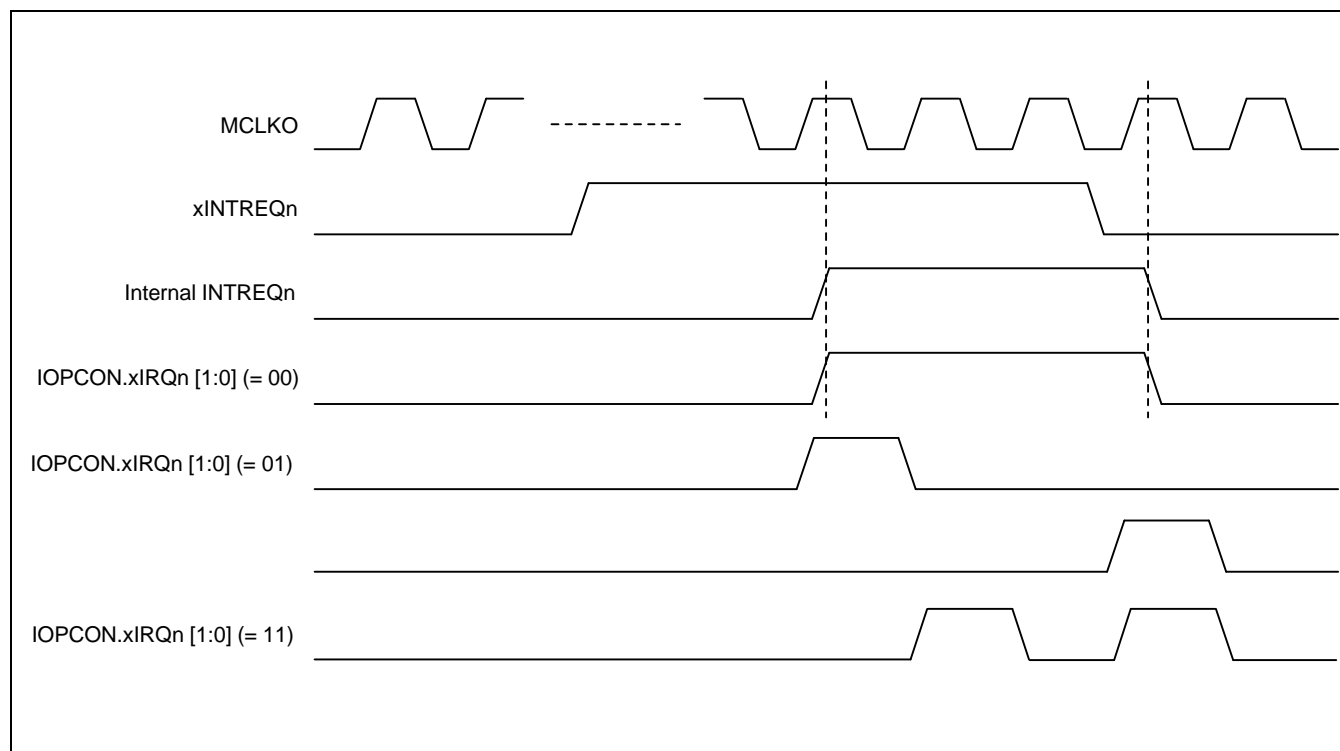
Figure 12-5. External Interrupt Request Timing (Active High)
