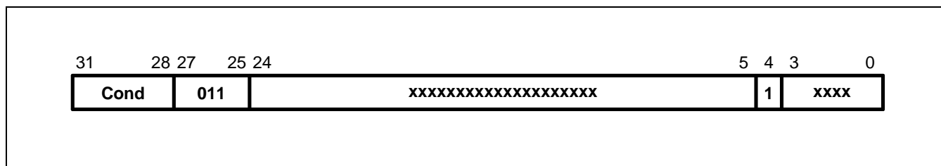
Figure 3-28. Undefined Instruction
