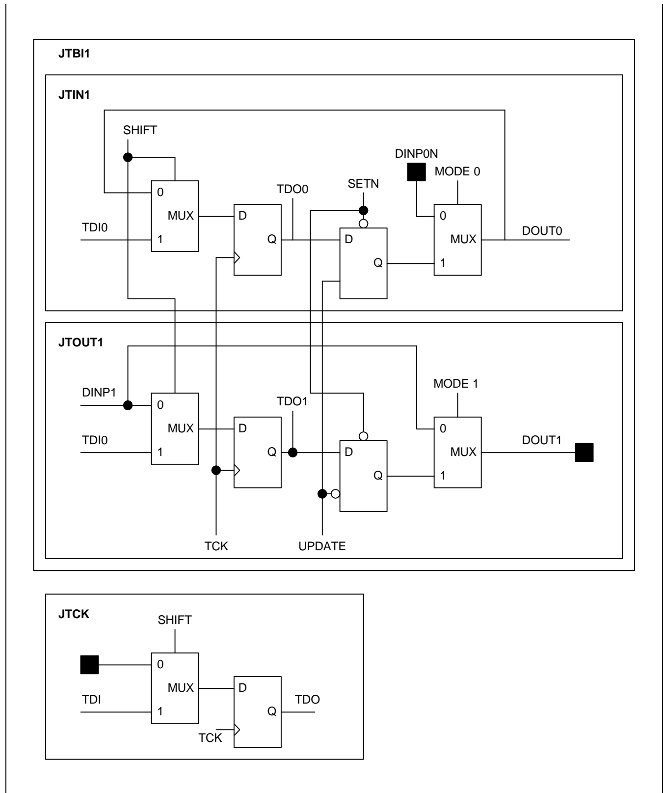
Figure A-2. S3C4510B Scan Cells
