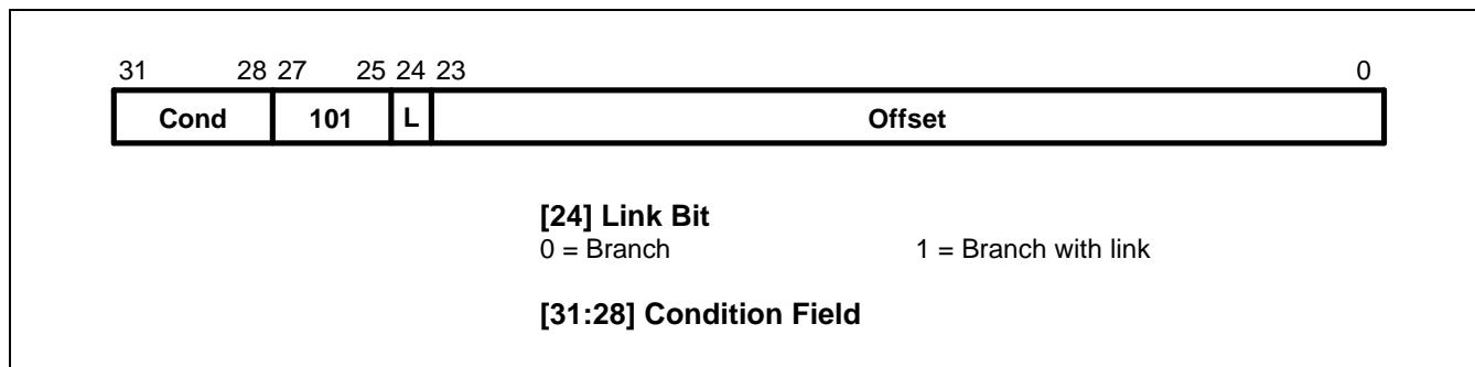
Figure 3-3. Branch Instructions
