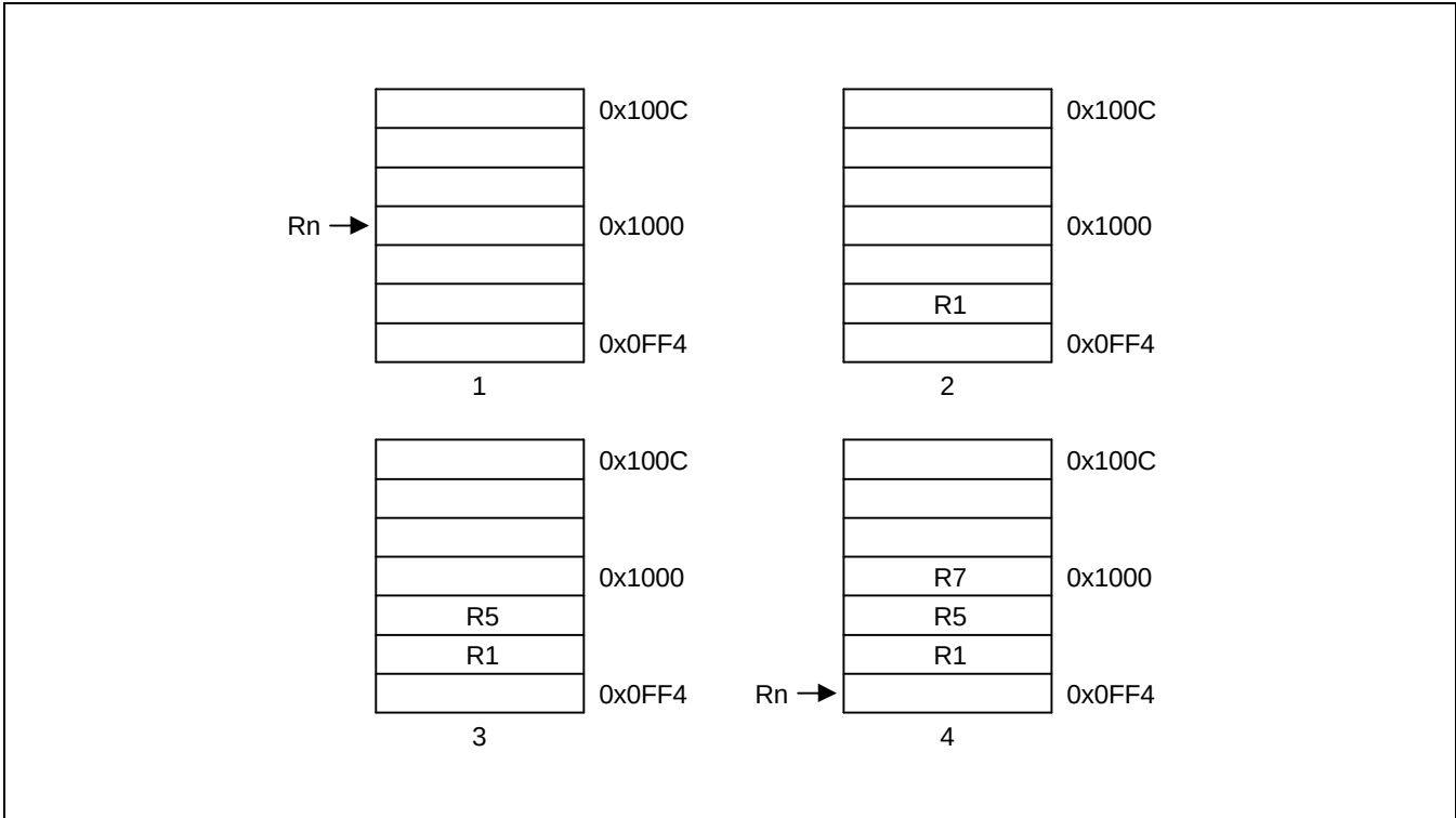
Figure 3-21. Post-Decrement Addressing
