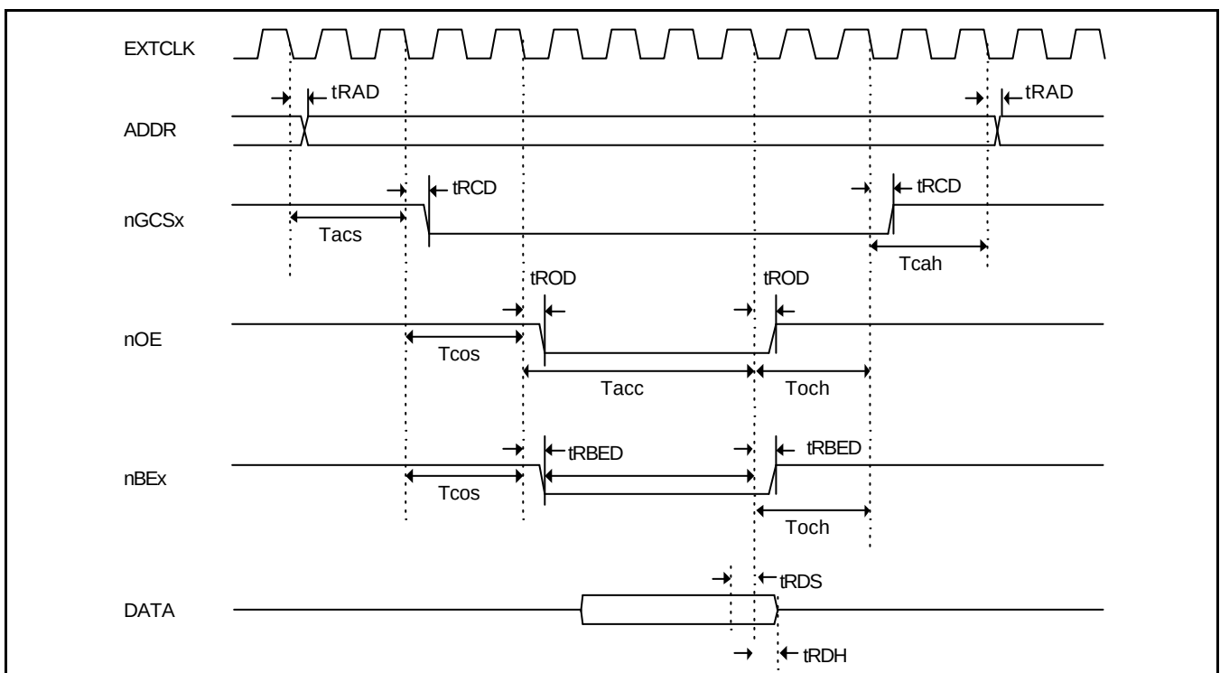
Figure 19-13. ROM/SRAM READ Timing (II) ( T_{acs}=2, T_{cos}=2, T_{acc}=4, T_{och}=2, T_{cah}=2\text{cycle}, PMC=0, ST=1 )
