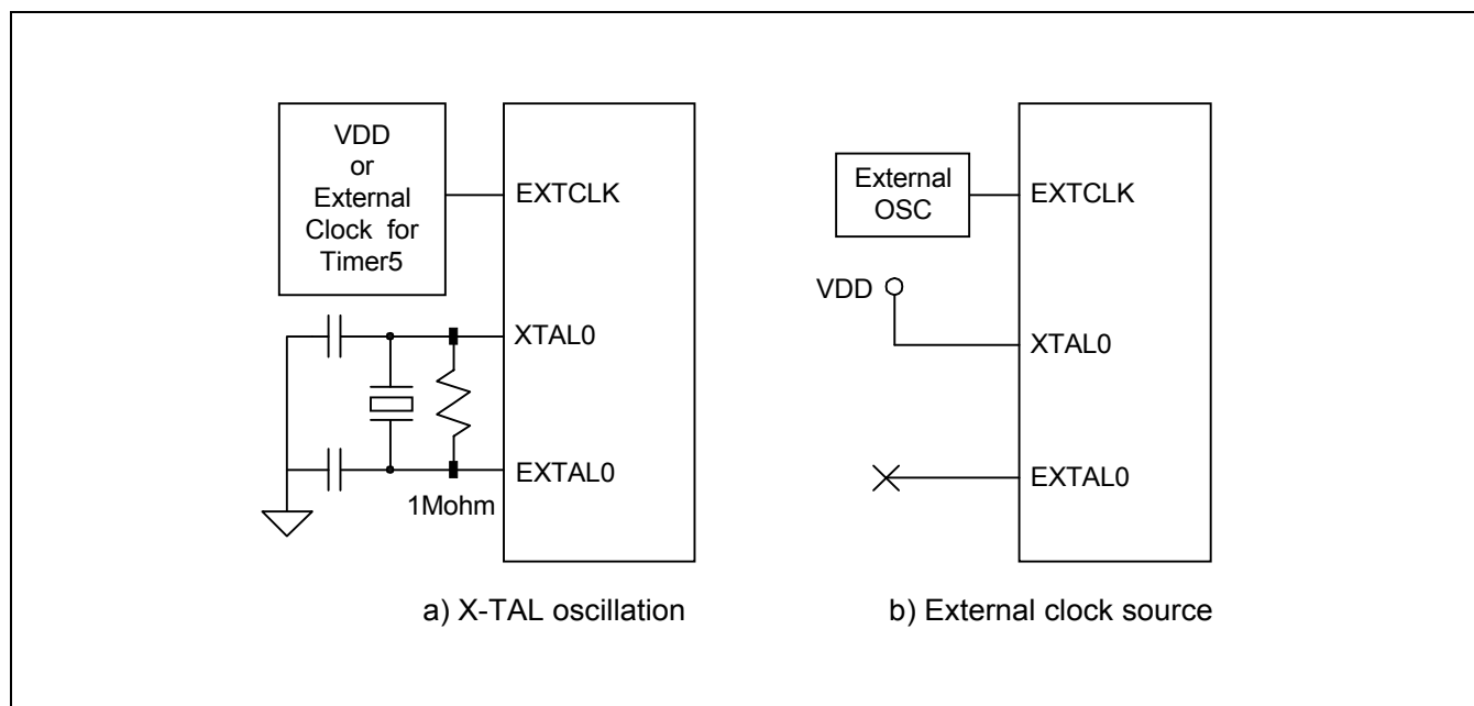
Figure 5-3. Main Oscillator Circuit Examples
