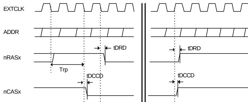
Figure 19-24. DRAM Self Refresh Timing
