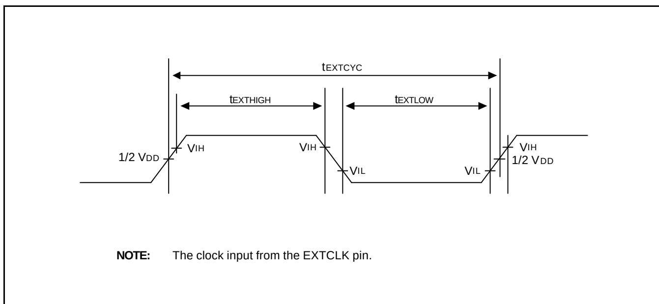
Figure 19-3. EXTCLK Clock Input Timing
