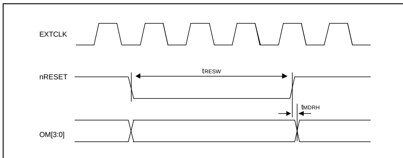
Figure 19-6. Manual Reset and OM[3:0] Input Timing
