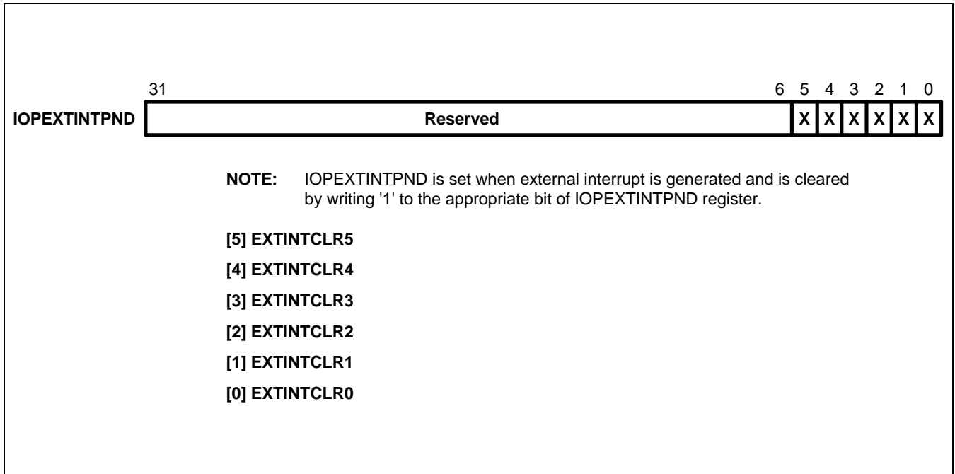
Figure 12-6. I/O Port External Interrupt Clear Register (IOEXTINTPND)
