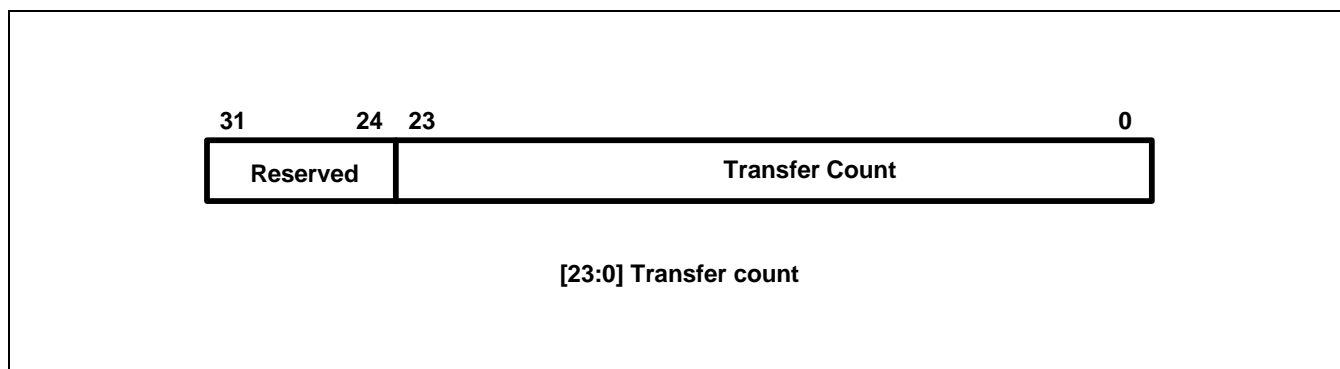
Figure 9-5. GDMA Transfer Count Register
