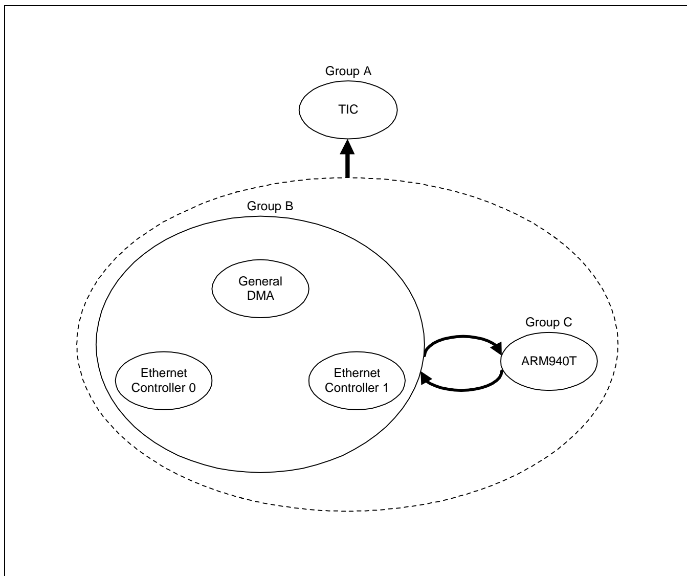
Figure 4-3. Priority Groups of S3C2501X
