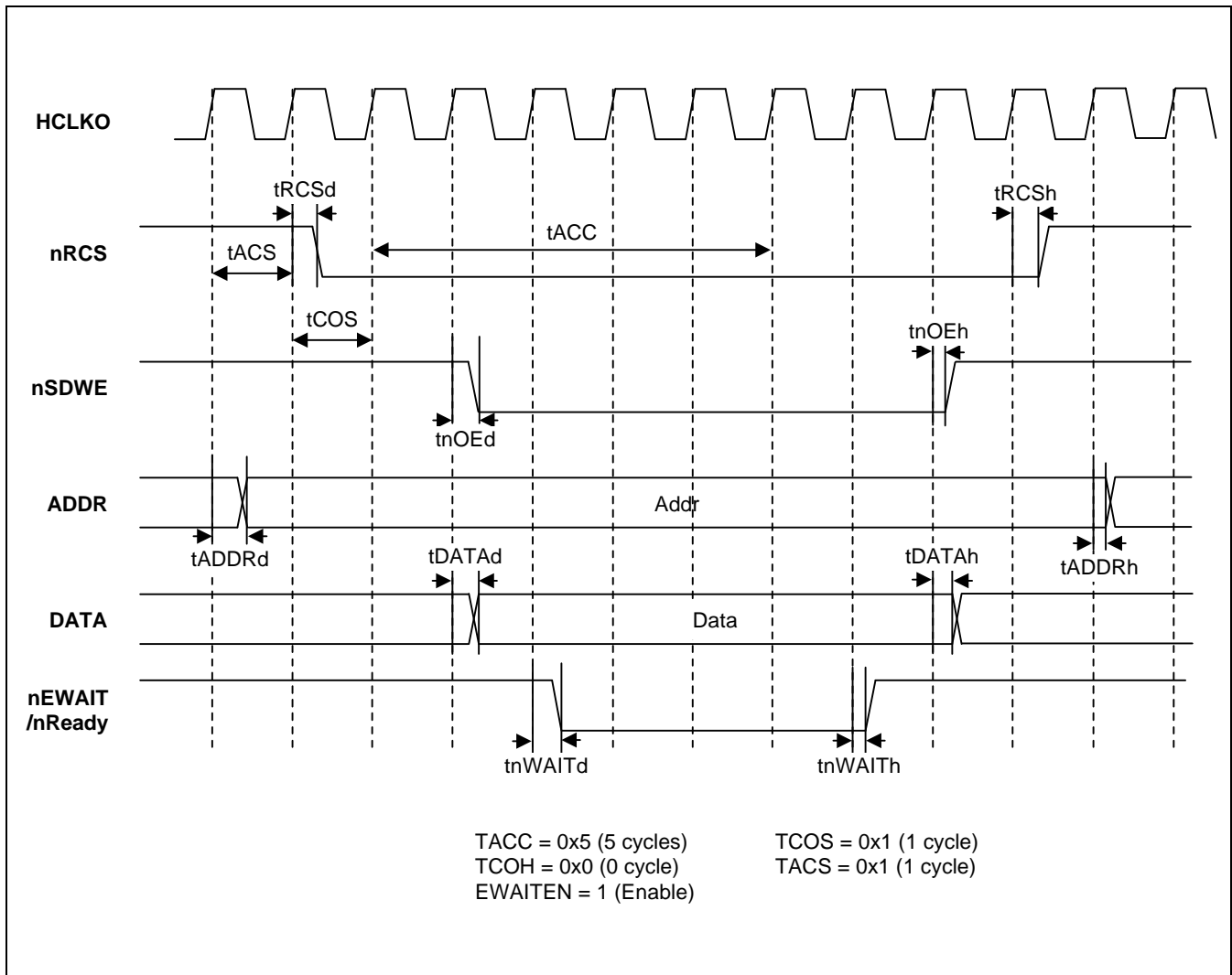
Figure 5-21. Write Timing Diagram (nEWAIT)
