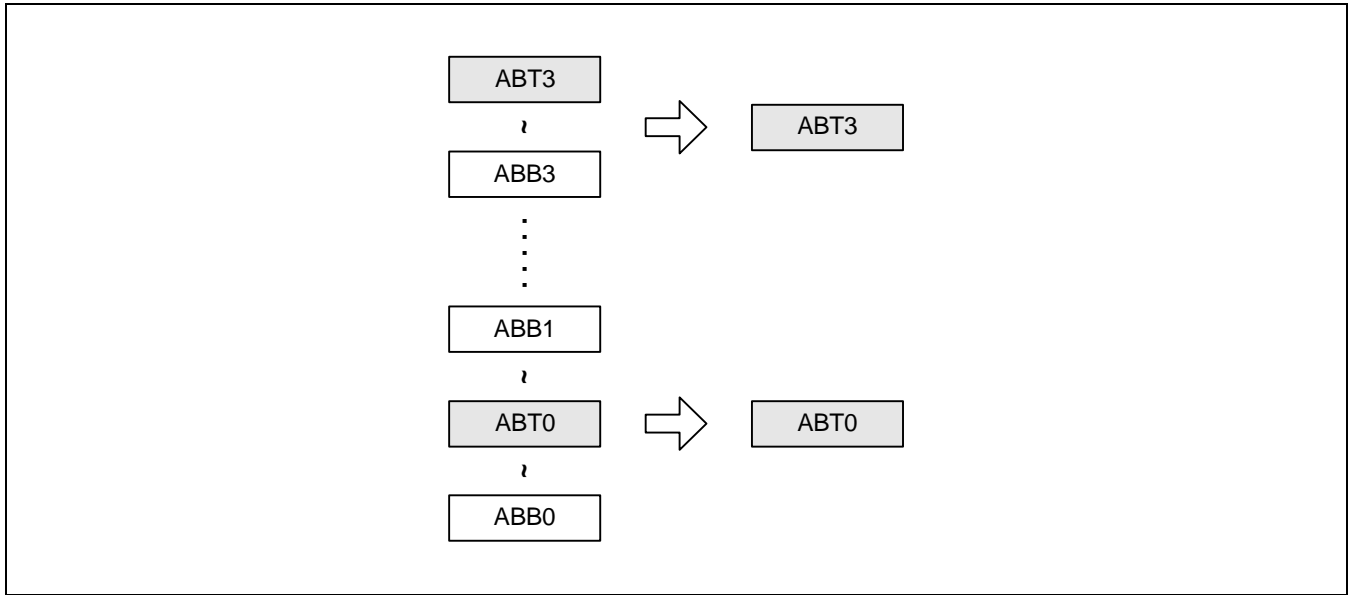
Figure 11-11. AutoBaud Boundary Register Range
