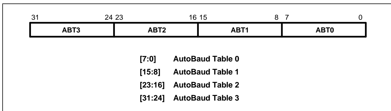
Figure 11-14. High-Speed UART AutoBaud Table Register
