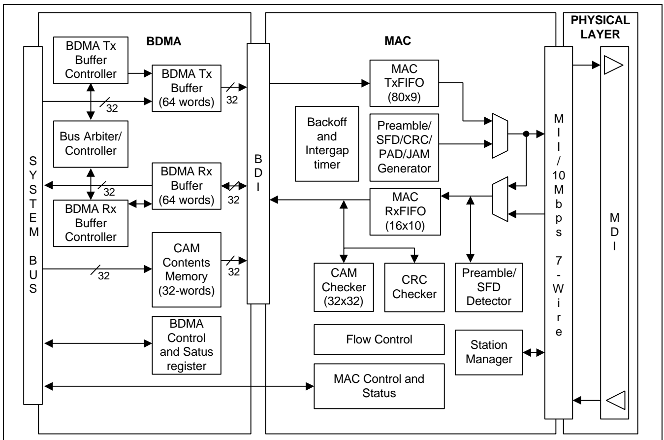
Figure 7-1. Ethernet Diagram
