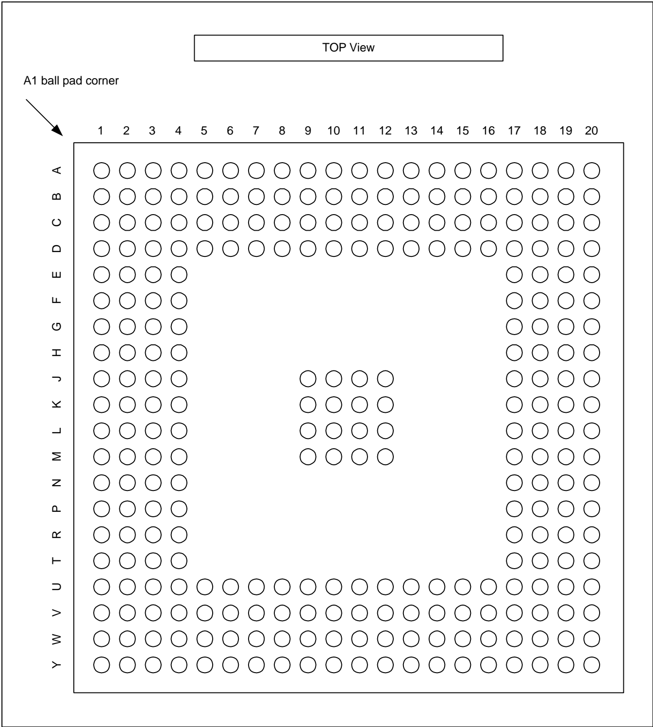
Figure 1-2. S3C2501X Pin Assignment Diagram
