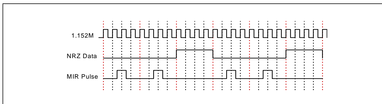
Figure 12-4. Pulse Modulation in MIR Mode
