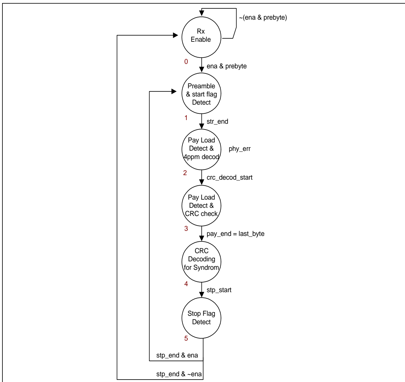
Figure 12-3. Fir Demodulation Process
