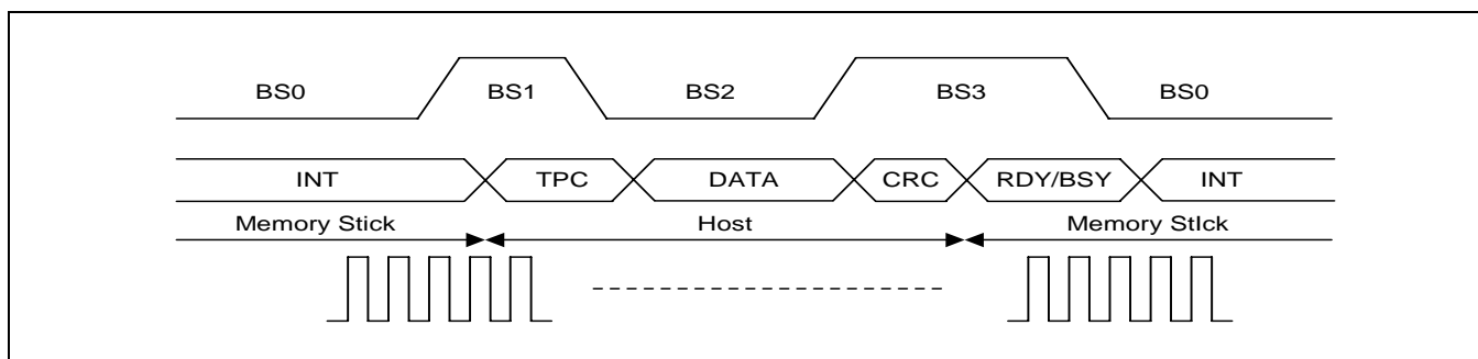
Figure 32-1. Memory Stick Write Packet
