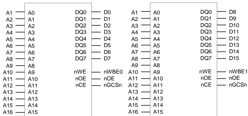
Figure 5-5. Memory Interface with 8-bit ROM x 2
