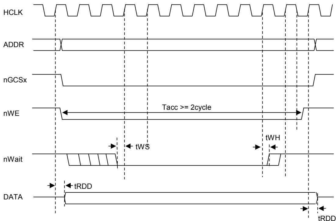
Figure 25-17. External nWAIT WRITE Timing (Tacs=0, Tcos=0, Tacc=4, Toch=0, Tcah=0, PMC=0, ST=0)
