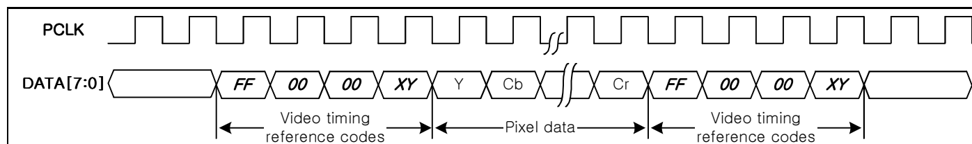
Figure 23-3. ITU-R BT.656 Input timing diagram
