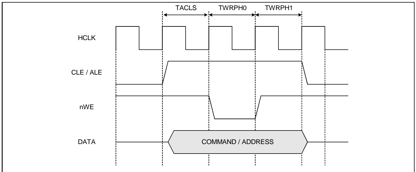
Figure 6-3. CLE &amp; ALE Timing (TACLS=1, TWRPH0=0, TWRPH1=0)
