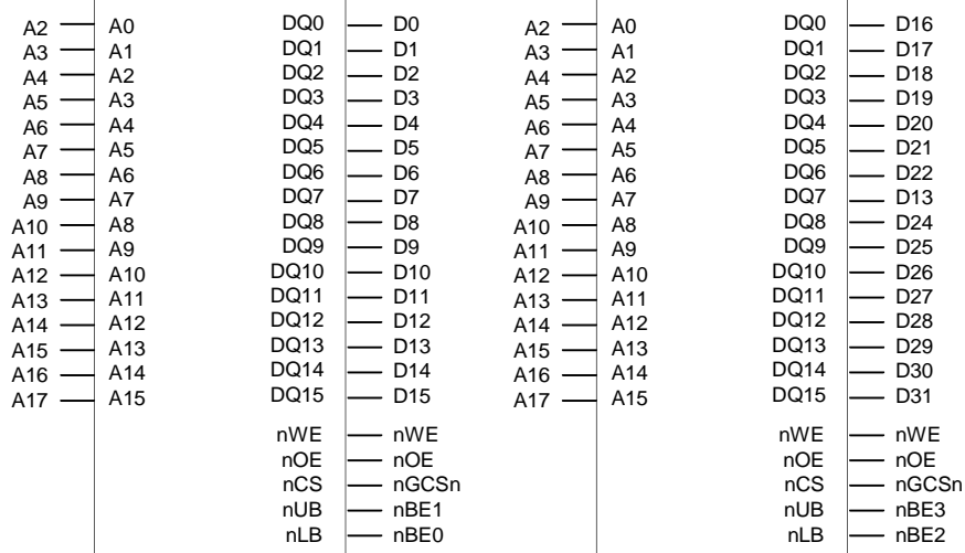
Figure 5-9. Memory Interface with 16-bit SRAM x 2
