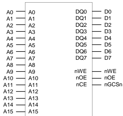
Figure 5-4. Memory Interface with 8-bit ROM
