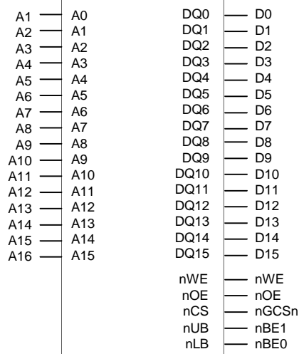
Figure 5-8. Memory Interface with 16-bit SRAM
