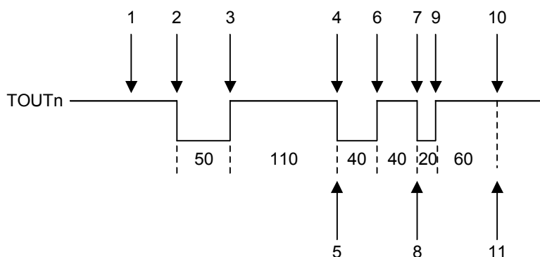
Figure 10-4. Example of a Timer Operation
