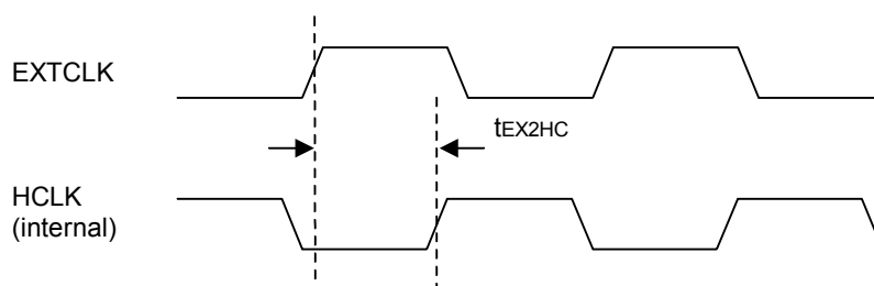
Figure 25-4. EXTCLK/HCLK in case that EXTCLK is used without the PLL
