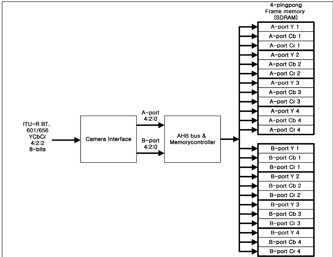
Figure 23-6. Ping-pong memory hierarchy
