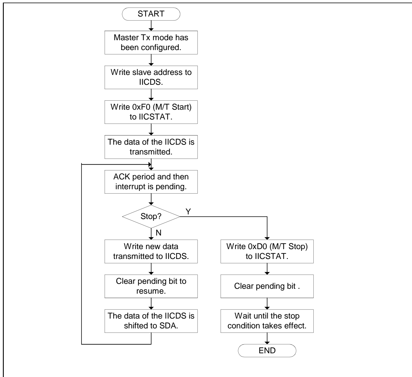
Figure 20-6 Operations for Master/Transmitter Mode
