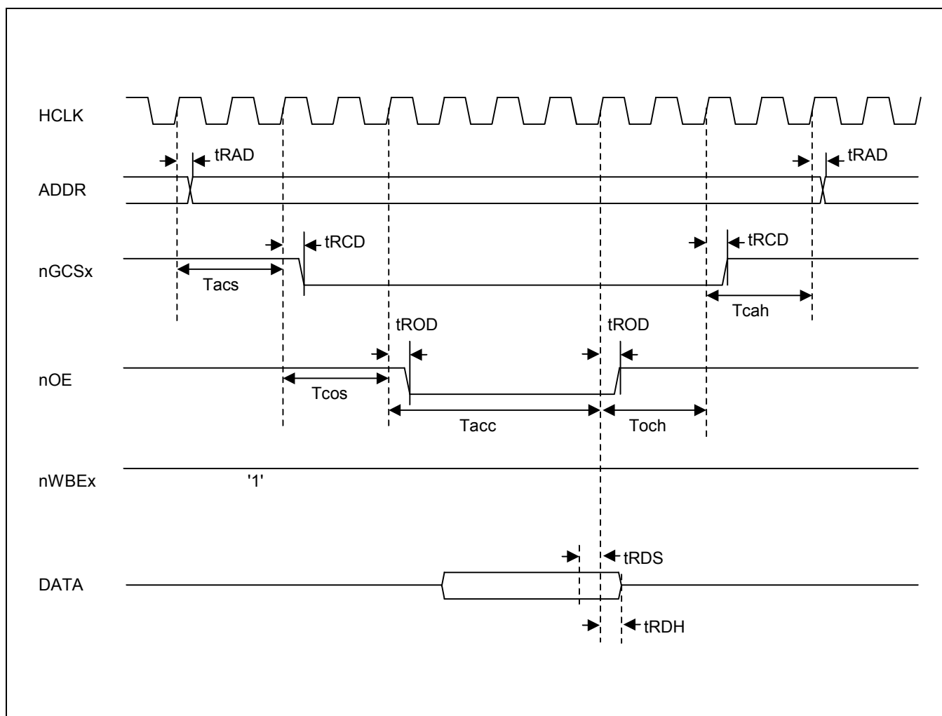
Figure 25-12. ROM/SRAM READ Timing (I) ( T_{acs}=2, T_{cos}=2, T_{acc}=4, T_{och}=2, T_{cah}=2, PMC=0, ST=0 )
