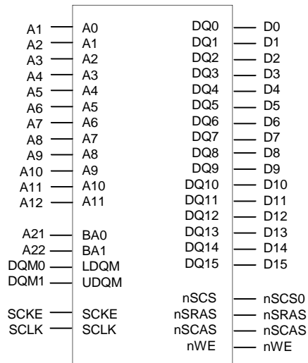
Figure 5-10. Memory Interface with 16-bit SDRAM (4Mx16, 4banks)
