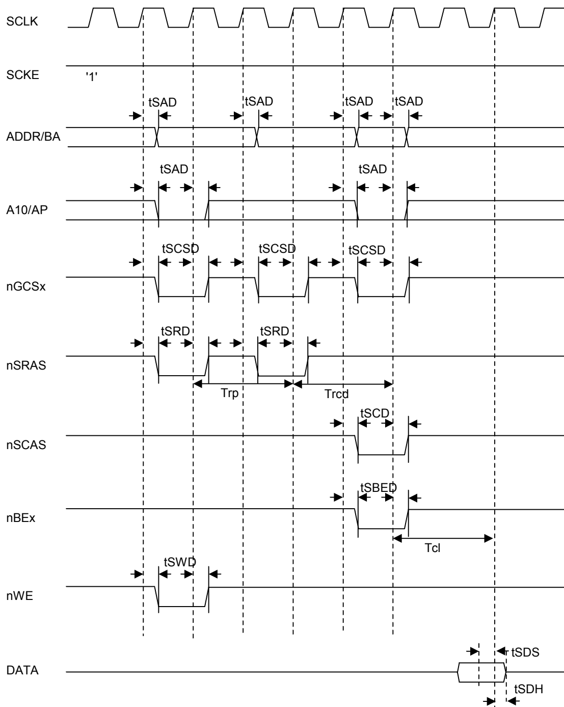
Figure 25-23. SDRAM Single READ Timing(I) ( Trp=2 , Trcd=2 , Tcl=2 )
