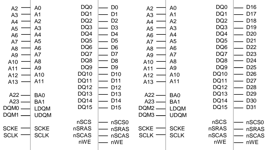
Figure 5-11. Memory Interface with 16-bit SDRAM (4Mx16 * 2ea, 4banks)
