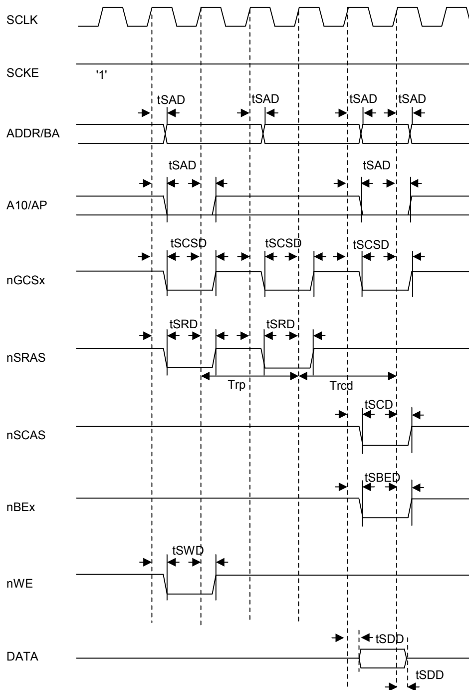
Figure 25-28. SDRAM Single Write Timing ( Trp=2 , Trcd=2 )
