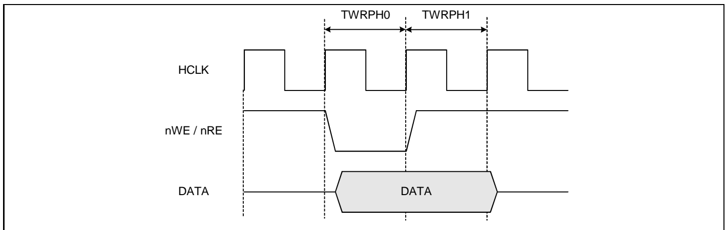
Figure 6-4 nWE &amp; nRE Timing (TWRPH0=0, TWRPH1=0)
