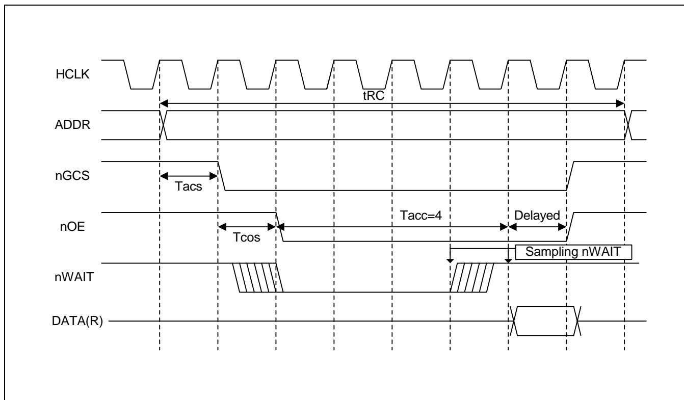
Figure 5-2. S3C2440X External nWAIT Timing Diagram ( T_{acc}=4 )
