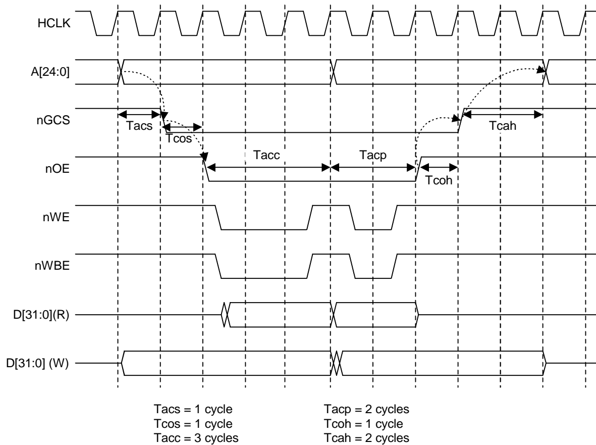
Figure 5-12. S3C2440X nGCS Timing Diagram
