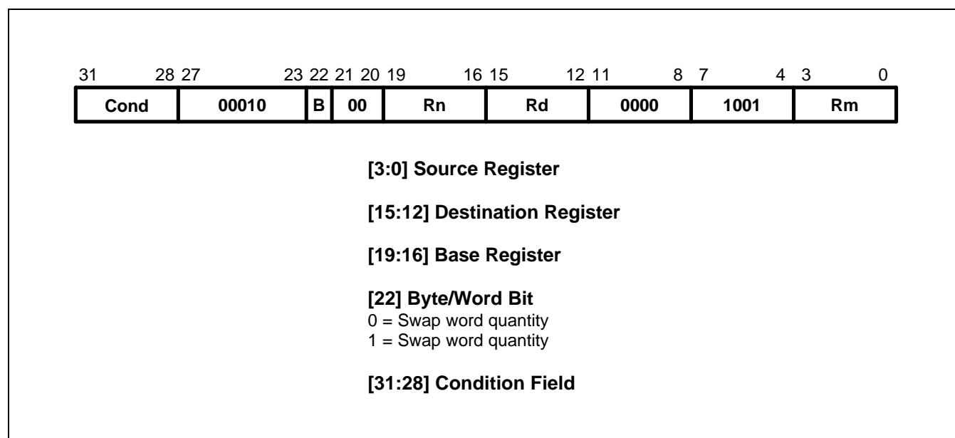
Figure 3-23. Swap Instruction
