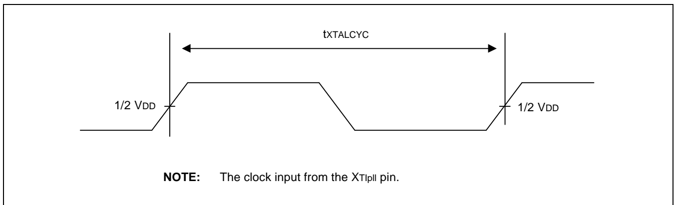
Figure 24-2. XTlpII Clock Timing
