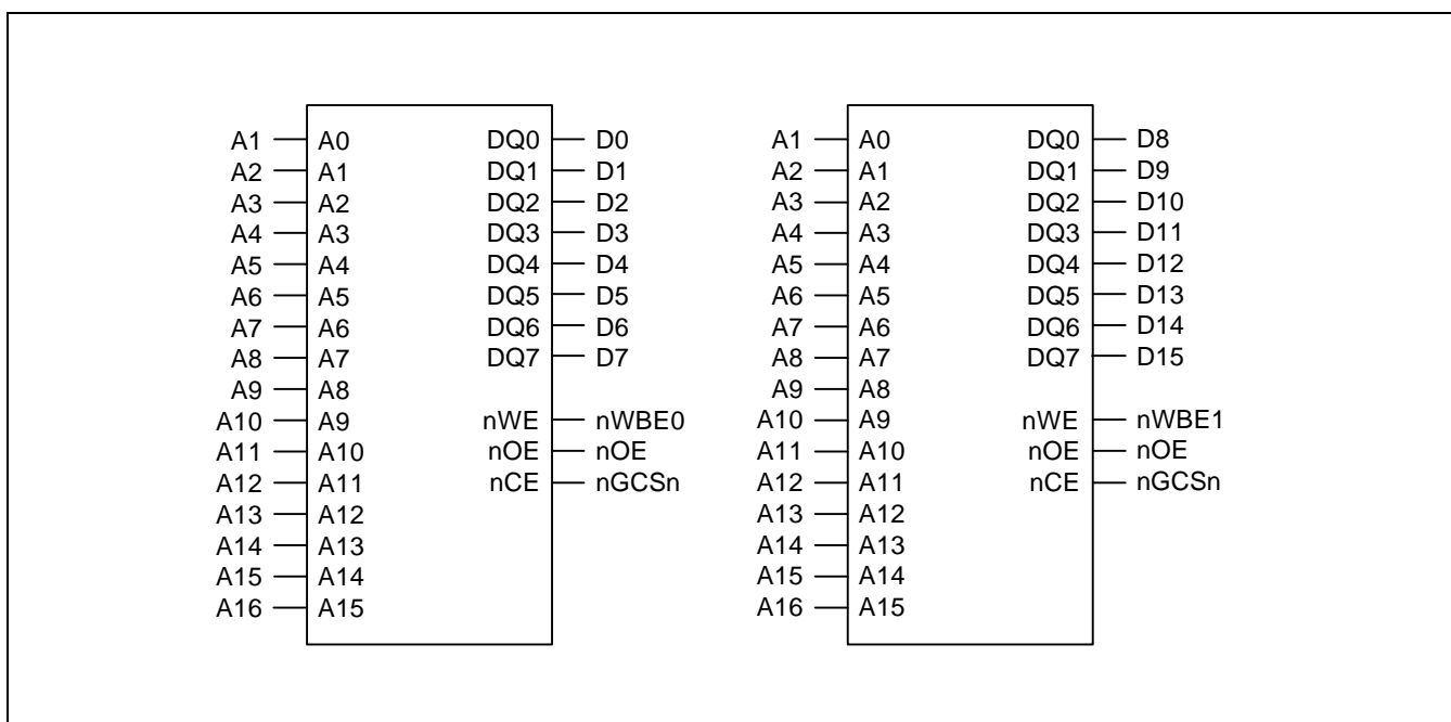
Figure 5-5. Memory Interface with 8-bit ROM × 2
