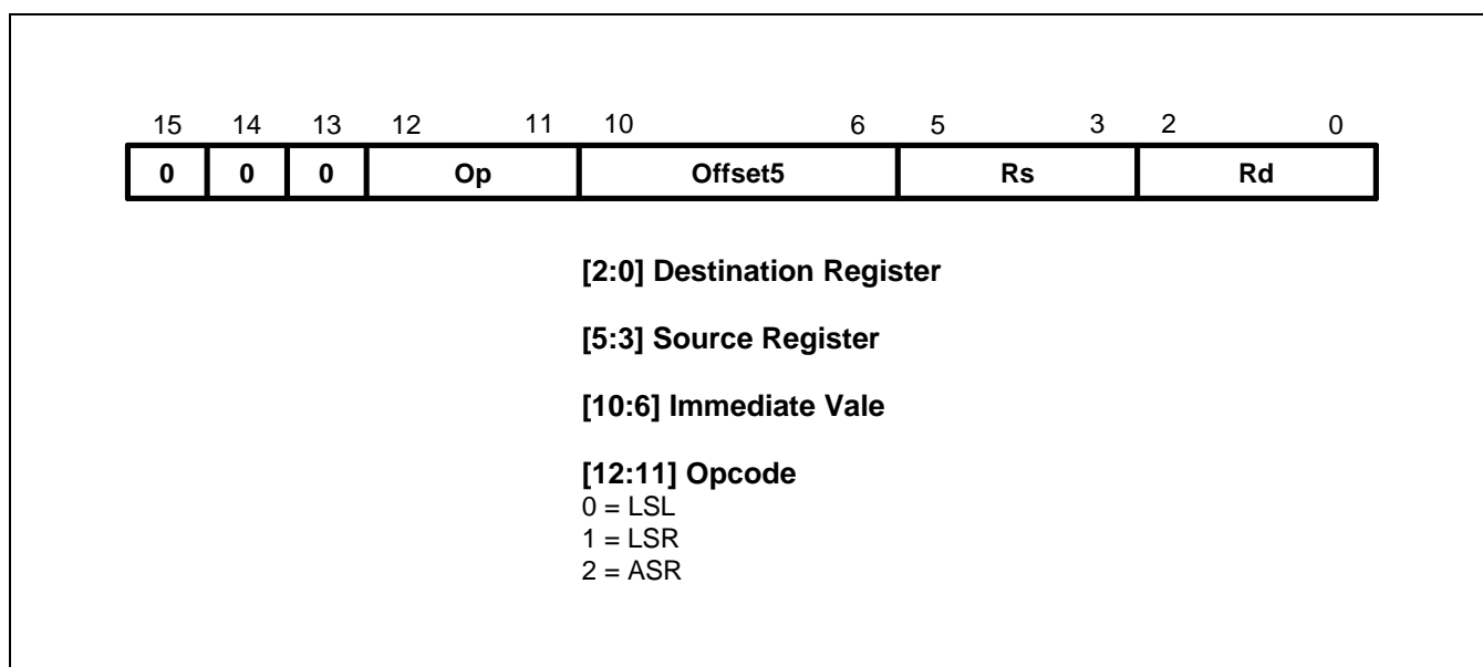
Figure 4-2. Format 1
