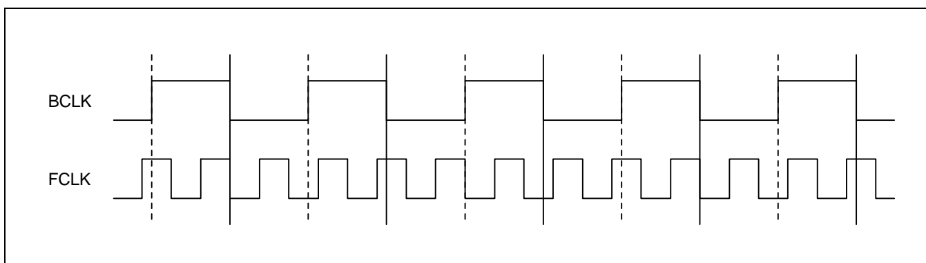
Figure 5-4. Asynchronous Clocking Mode
