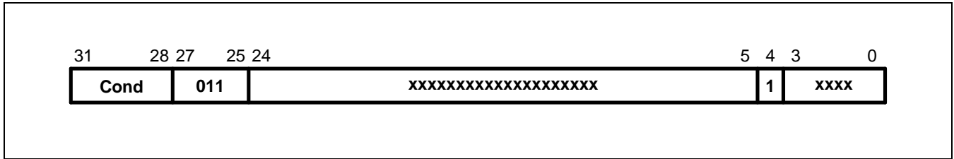
Figure 3-28. Undefined Instruction
