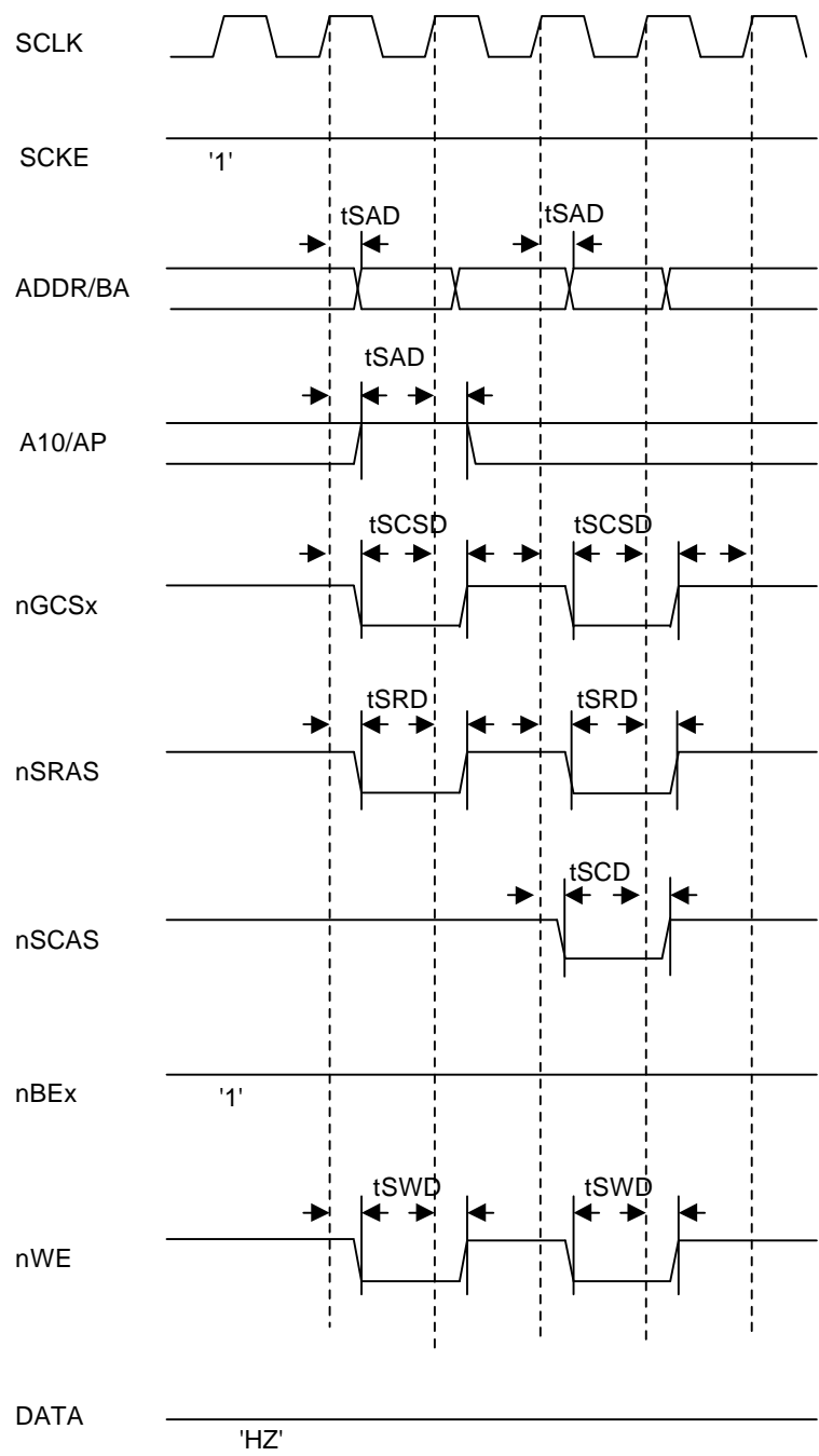
Figure 24-22. SDRAM MRS Timing
