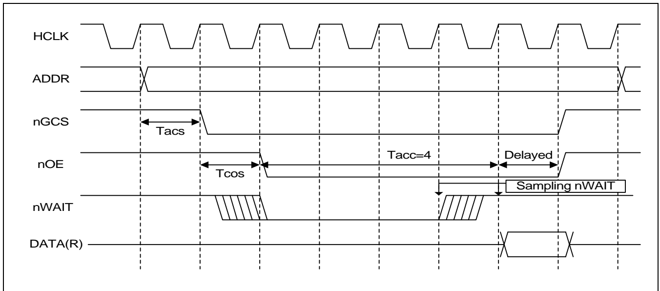
Figure 5-2. S3C2410X External nWAIT Timing Diagram ( T_{acc}=4 )
