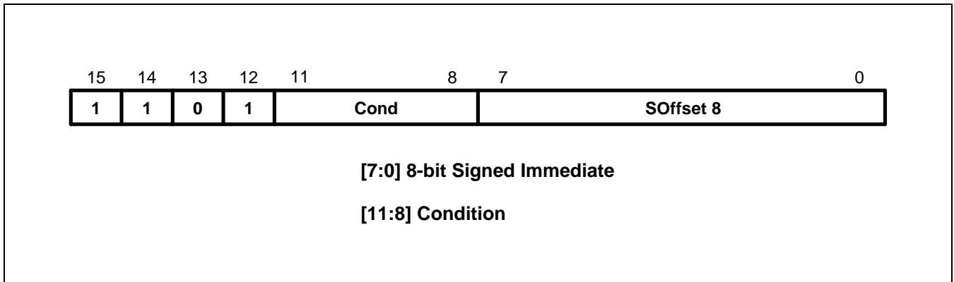
Figure 4-17. Format 16
