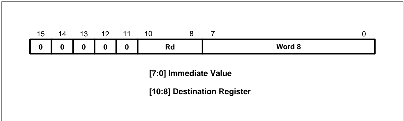
Figure 4-7. Format 6
