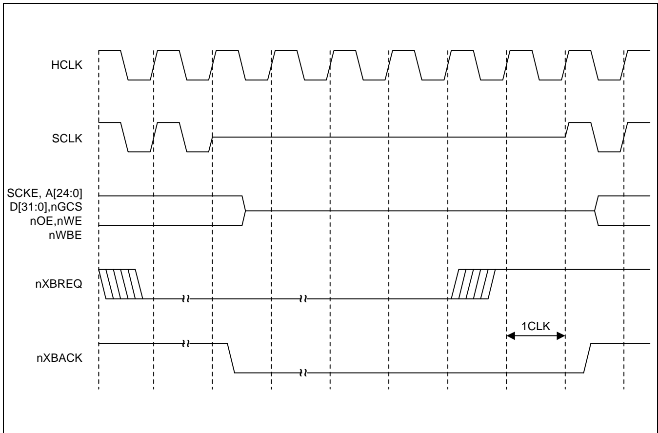
Figure 5-3. S3C2410X nXBREQ/nXBACK Timing Diagram
