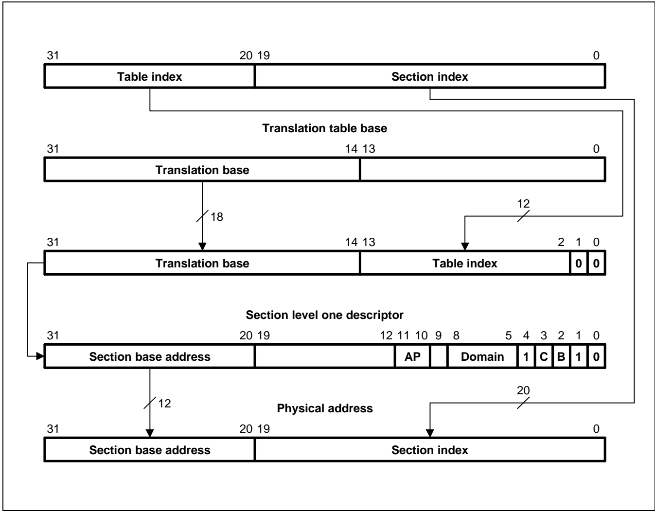
Figure 3-5. Section Translation
