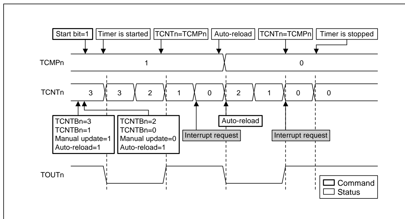
Figure 10-2. Timer Operations
