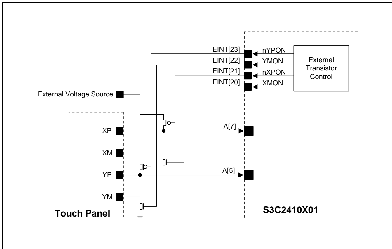
Figure 16-2. Example of ADC and Touch Screen Interface
