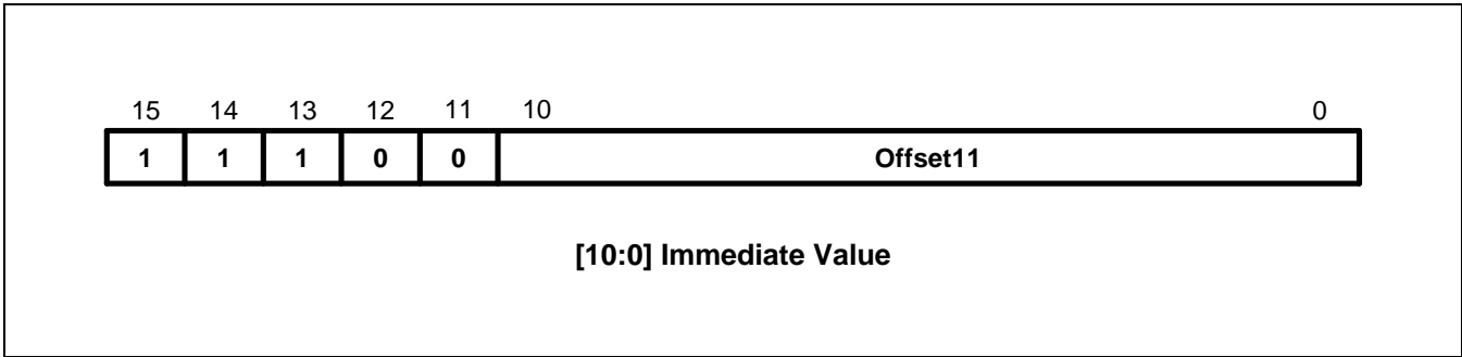
Figure 4-19. Format 18
