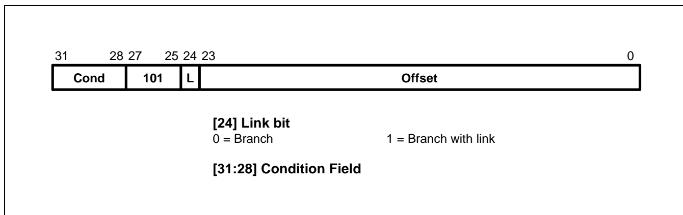
Figure 3-3. Branch Instructions
