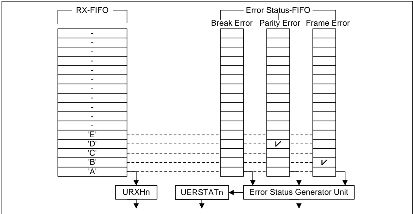
Figure 11-3. UART Receiving 5 Characters with 2 Errors
