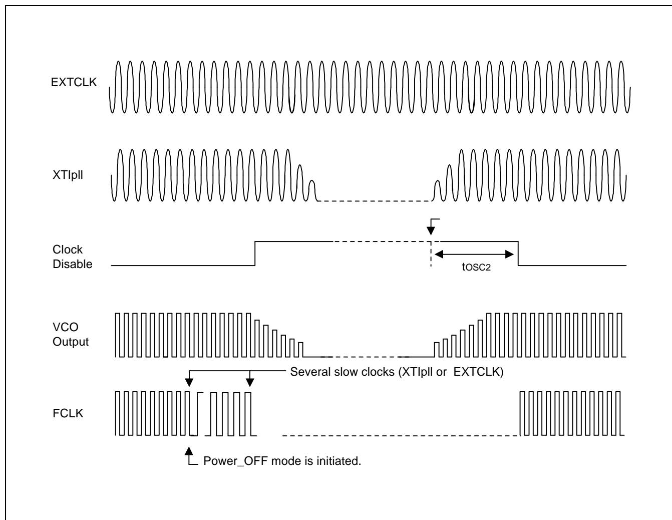
Figure 24-8. Power_OFF Mode Return Oscillation Setting Timing
