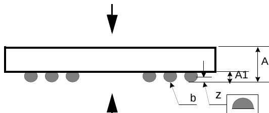
*1: Bottom View
