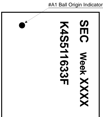
< Top View *2 >
