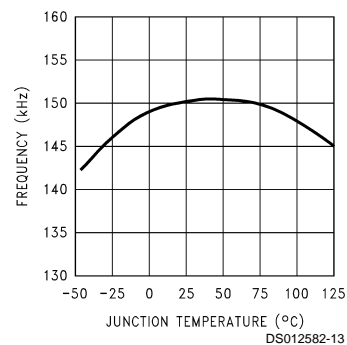
Switching Frequency
