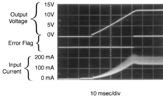
FIGURE 24. Output Voltage, Input Current, Error Flag Signal, at Start-Up, WITH Soft-start
