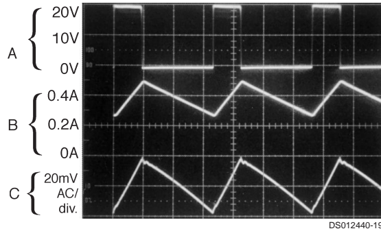
Continuous Mode Switching Waveforms
