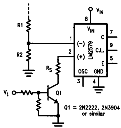
FIGURE 12. Remote Shutdown
