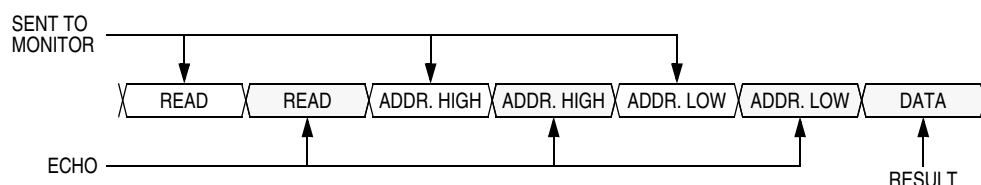
Figure 10-5. Read Transaction
