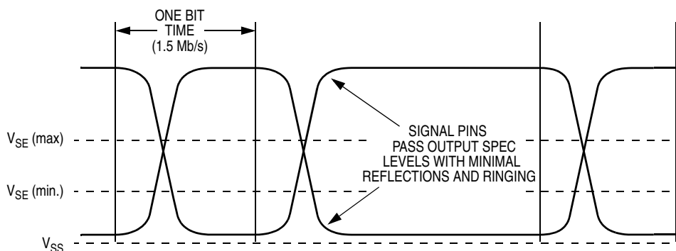
Figure 9-11. Receiver Characteristics
