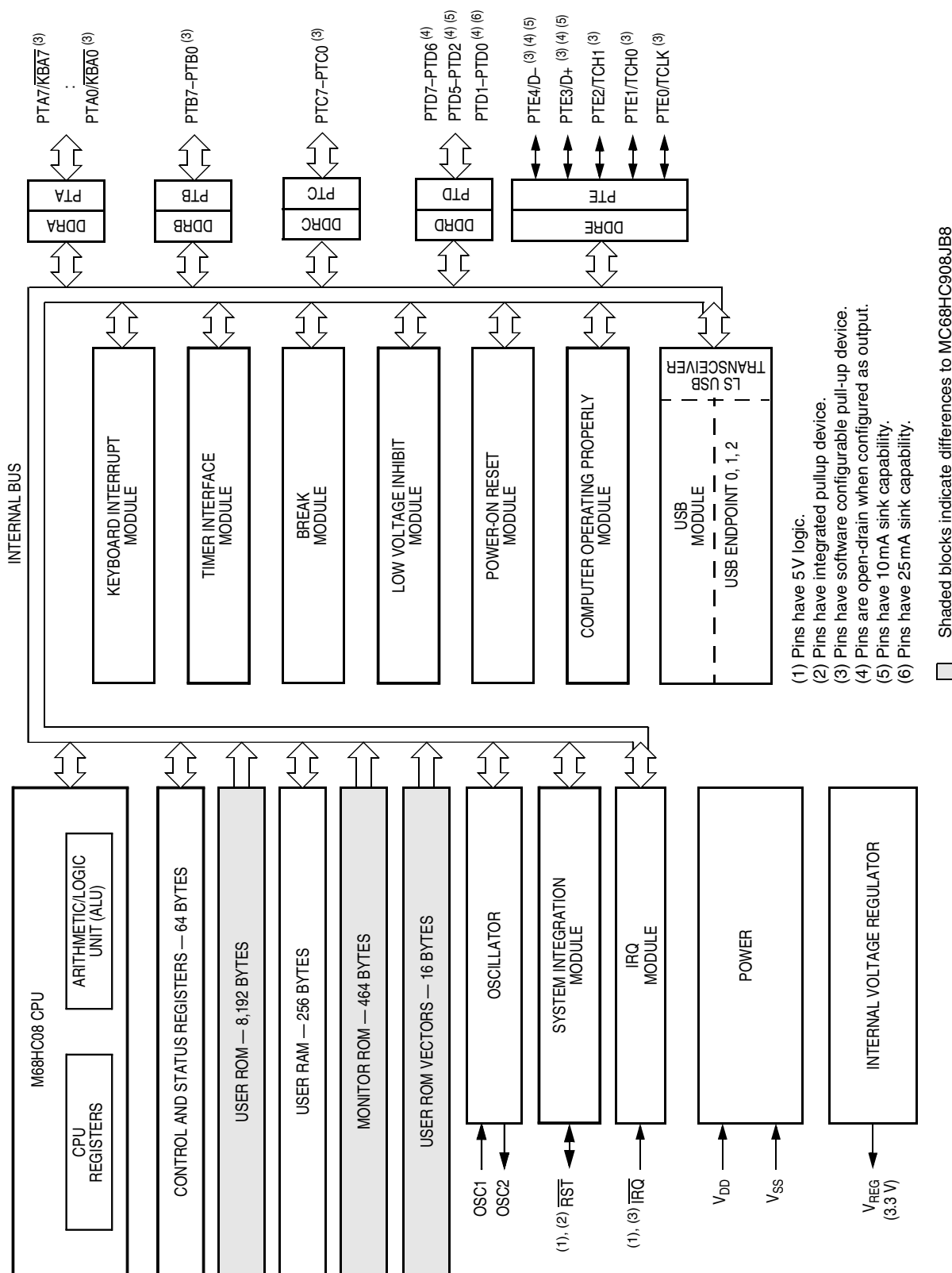
Figure A-1. MC68HC08JB8 Block Diagram
