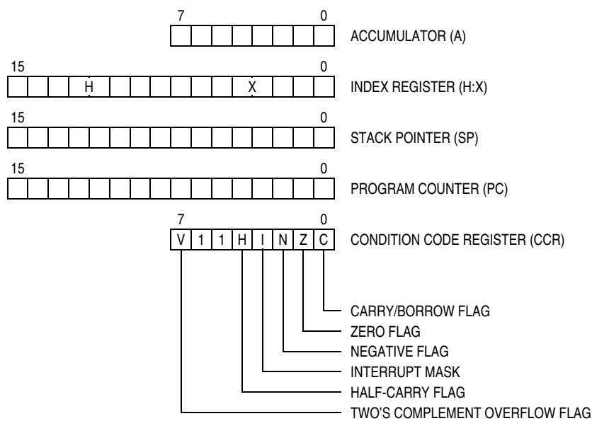
Figure 6-1. CPU Registers
