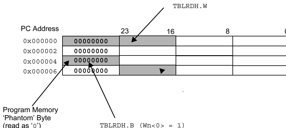
FIGURE 3-5: PROGRAM DATA TABLE ACCESS (MS BYTE)
