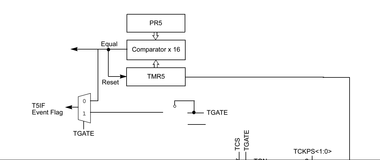
FIGURE 11-3: 16-BIT TIMER5 BLOCK DIAGRAM
