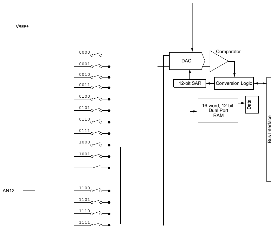
FIGURE 19-1: 12-BIT A/D FUNCTIONAL BLOCK DIAGRAM
