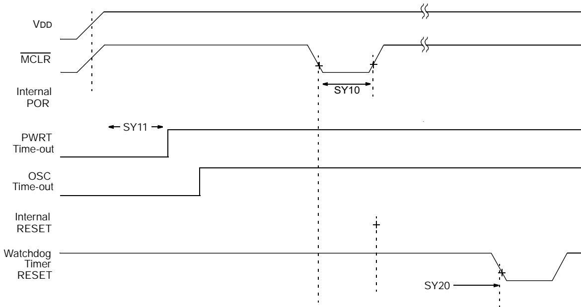
FIGURE 23-6: RESET, WATCHDOG TIMER, OSCILLATOR START-UP TIMER AND POWER-UP TIMER TIMING CHARACTERISTICS
