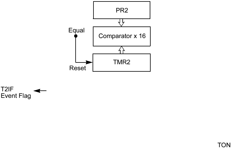
FIGURE 10-2: 16-BIT TIMER2 BLOCK DIAGRAM
