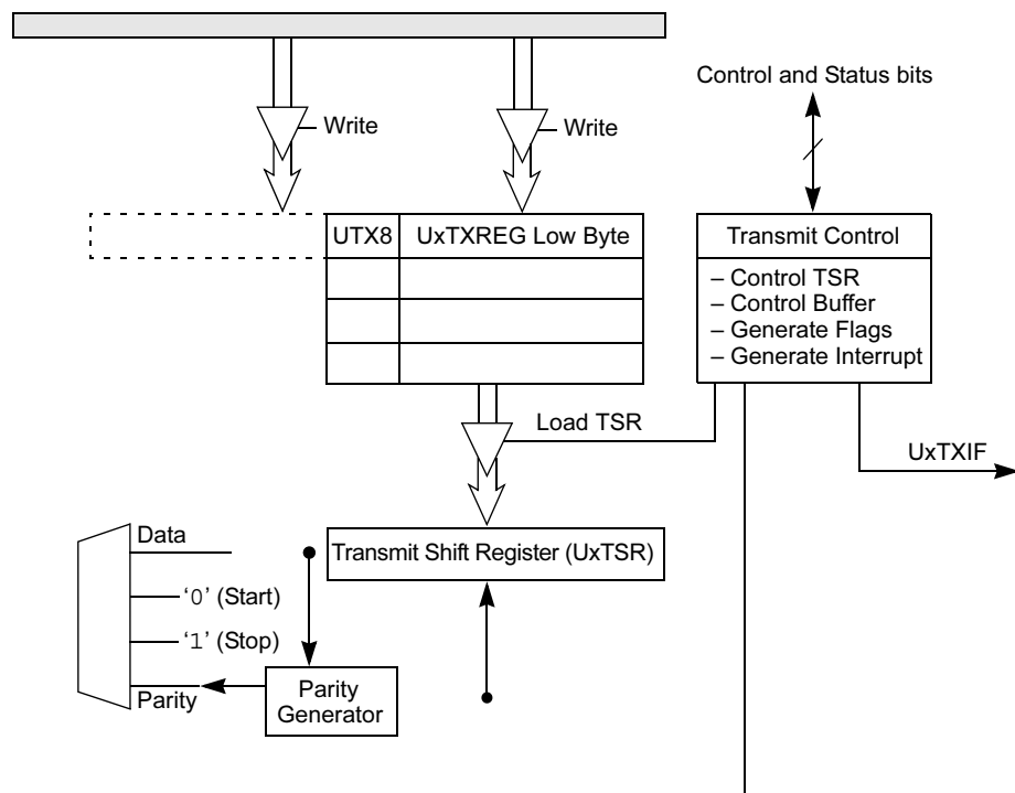
FIGURE 16-1: UART TRANSMITTER BLOCK DIAGRAM
