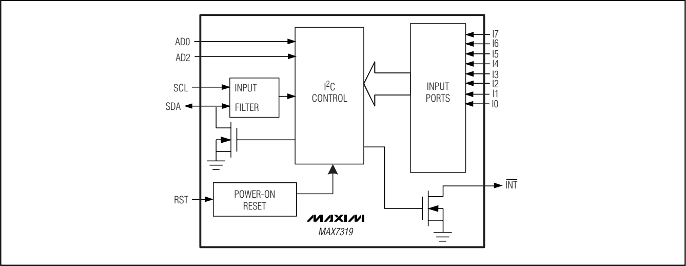
Functional Diagram
