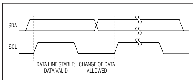
Figure 3. Bit Transfer
