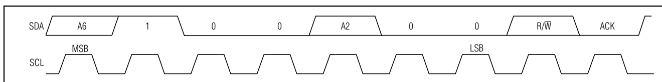
Figure 6. Slave Address
