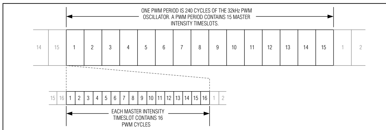
Figure 12. PWM Timing
