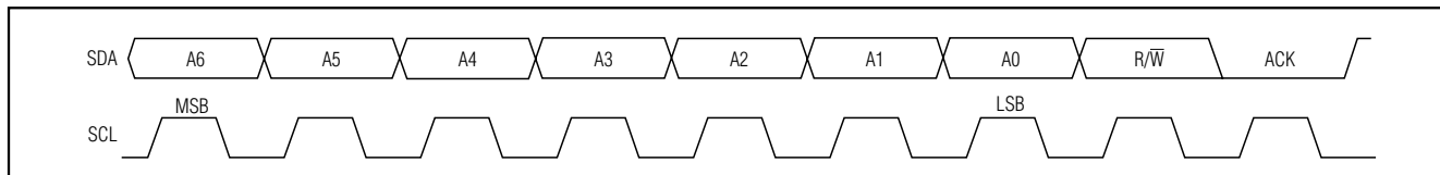
Figure 6. Slave Address
