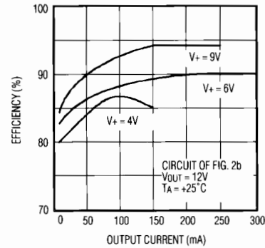
MAX752 EFFICIENCY vs. OUTPUT CURRENT
