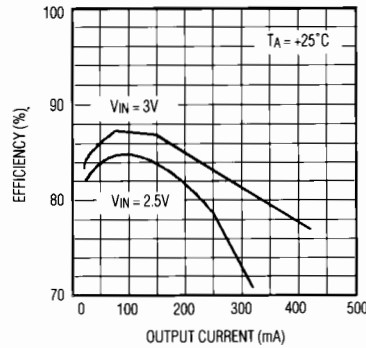
MAX731 EFFICIENCY vs. OUTPUT CURRENT
