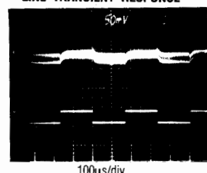
MAX752 LINE TRANSIENT RESPONSE
