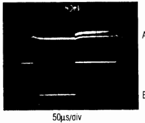
MAX752 LOAD TRANSIENT RESPONSE
