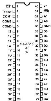
40 Lead DIP
