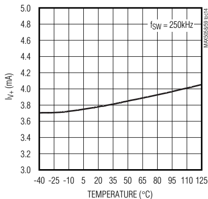
SWITCHING SUPPLY CURRENT vs. TEMPERATURE (MAX5058)
