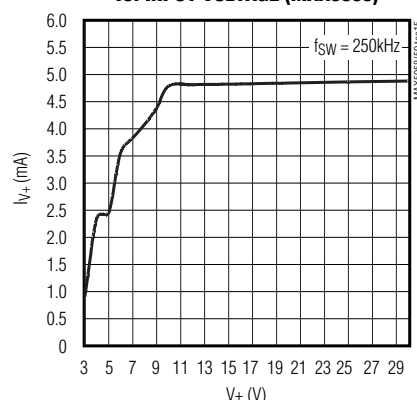
SWITCHING SUPPLY CURRENT vs. INPUT VOLTAGE (MAX5059)
