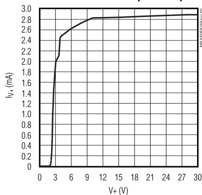
SWITCHING SUPPLY CURRENT vs. INPUT VOLTAGE (MAX5058)
