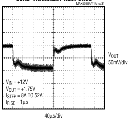
LOAD-TRANSIENT RESPONSE
