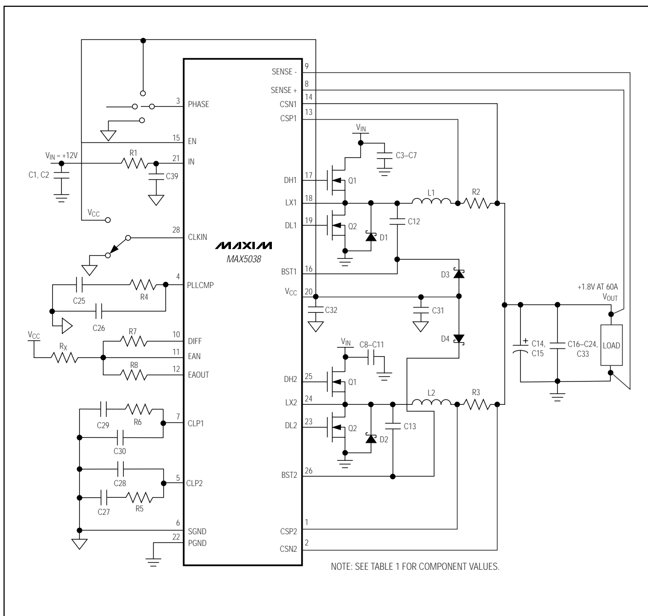
Figure 1. MAX5038 Typical Application Circuit, V_{IN} = +12V
