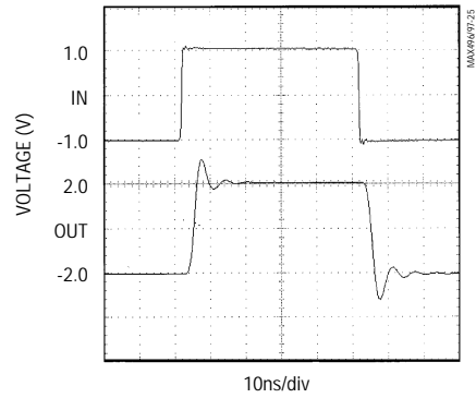
MAX497 LARGE-SIGNAL PULSE RESPONSE ( C_L = 47pF )
