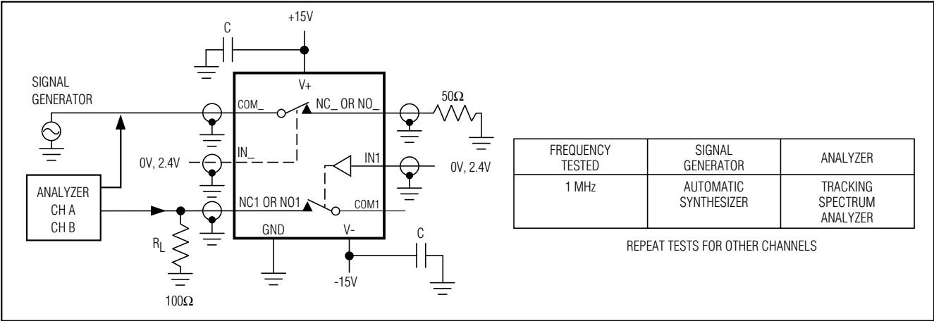
Figure 8. Crosstalk
