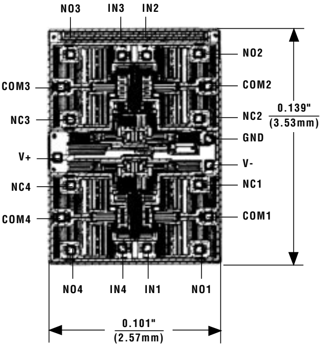
Chip Topography
