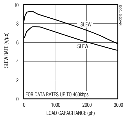
MAX3318/MAX3319 SLEW RATE vs. LOAD CAPACITANCE
