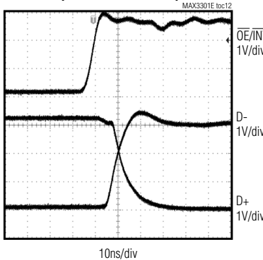
DRIVER DISABLE DELAY (FULL-SPEED MODE)
