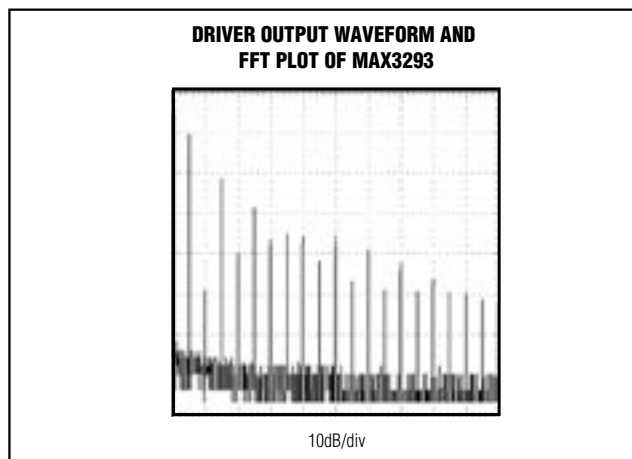
Figure 13. Driver Output Waveform and FFT Plot of MAX3293 Transmitting a 125kHz Signal
