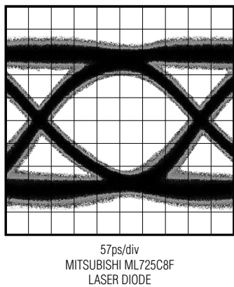
OPTICAL EYE DIAGRAM (2.488Gbps, 1300nm FP LASER, 1.87GHz FILTER)
