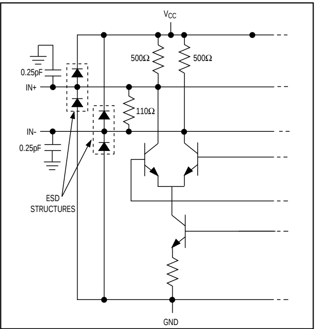
Figure 4. Input Circuit
