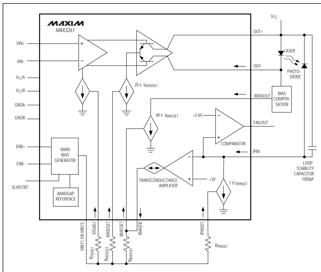
Figure 1. Functional Diagram
