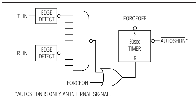
Figure 2c. AutoShutdown Plus Logic
