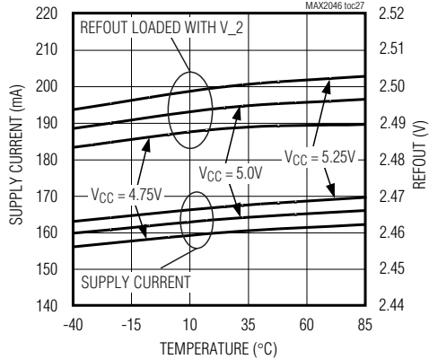
REFOUT AND SUPPLY CURRENT vs. TEMPERATURE AND SUPPLY VOLTAGE
