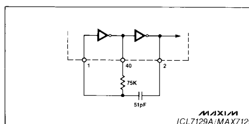
Figure 5B. RC Oscillator Circuit
