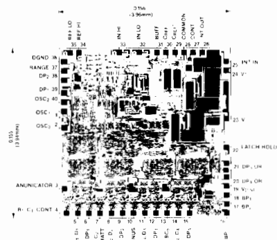
Substrate is Connected to V I .
