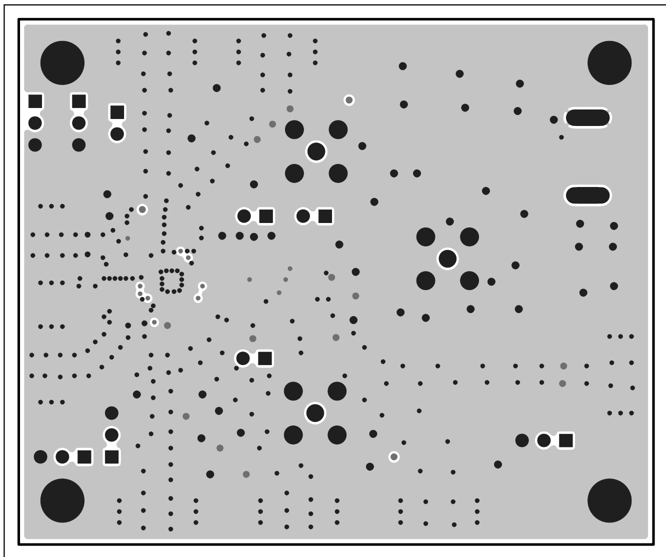
Figure 4. MAX2335 EV Kit PC Board Layout—Ground Layer 3
