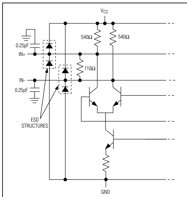
Figure 3. Input Circuit
