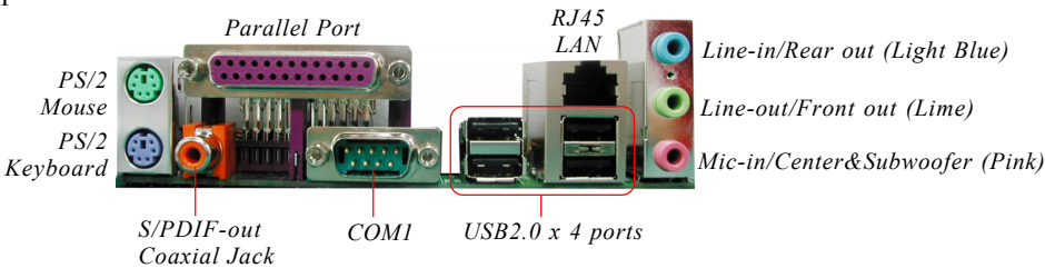
Figure 8 - I/O Ports
